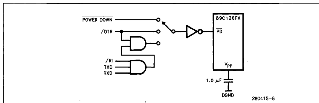
Figure 6. Power-Down Control
