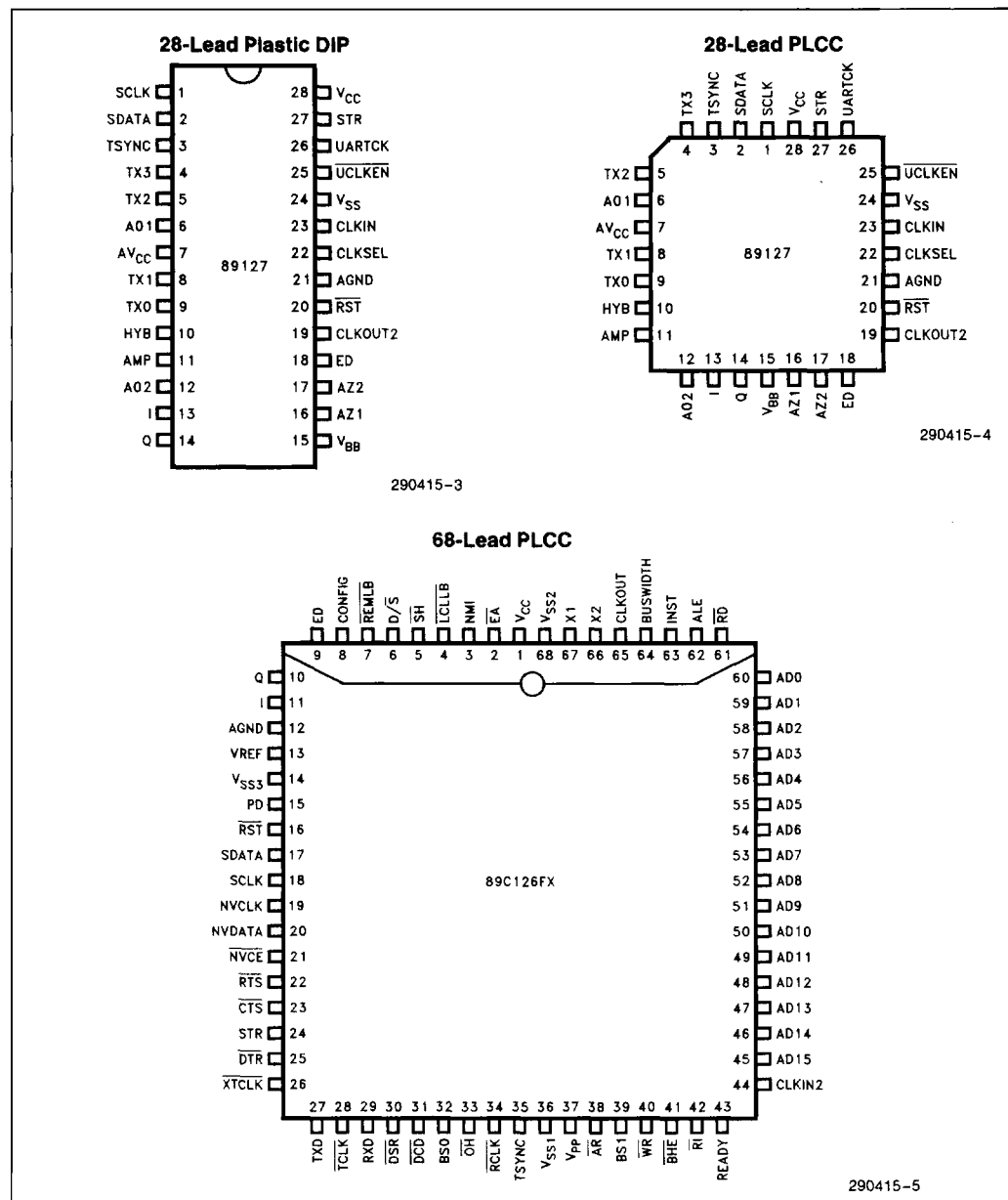
Figure 3. Device Packages
