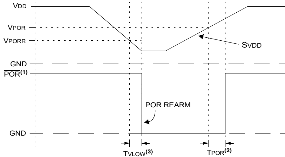
Figure 37-1. \overline{\text{POR}} and \overline{\text{POR}} Rearm with Slow Rising V_{DD}
