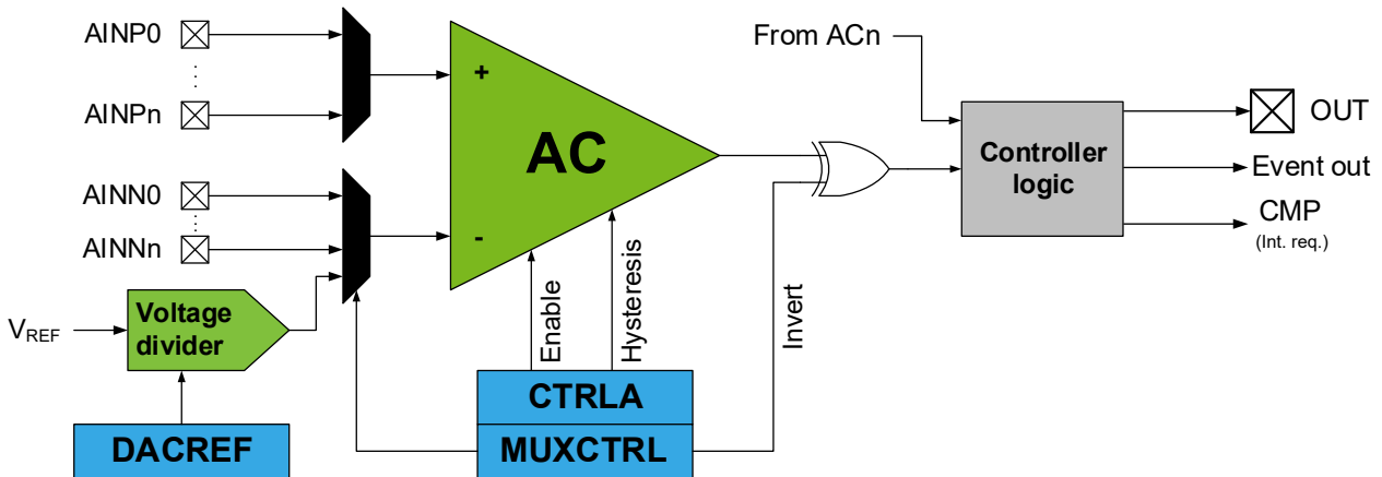
Figure 30-1. Analog Comparator
