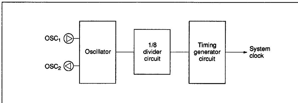
Figure 15 Internal Oscillator Circuit
