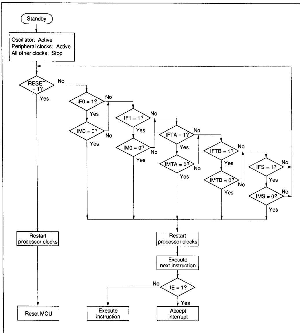
Figure 18 MCU Operating Flowchart in Standby Mode
