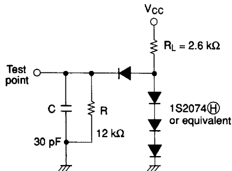
Figure 29 Timing Load Circuit
