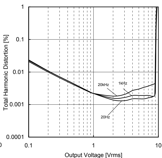
Figure 21. Total Harmonic Distortion vs Output Voltage (VCC/VEE=+15V/-15V, A v =20dB R L =600Ω, 80kHz-LPF, T A =25°C)
