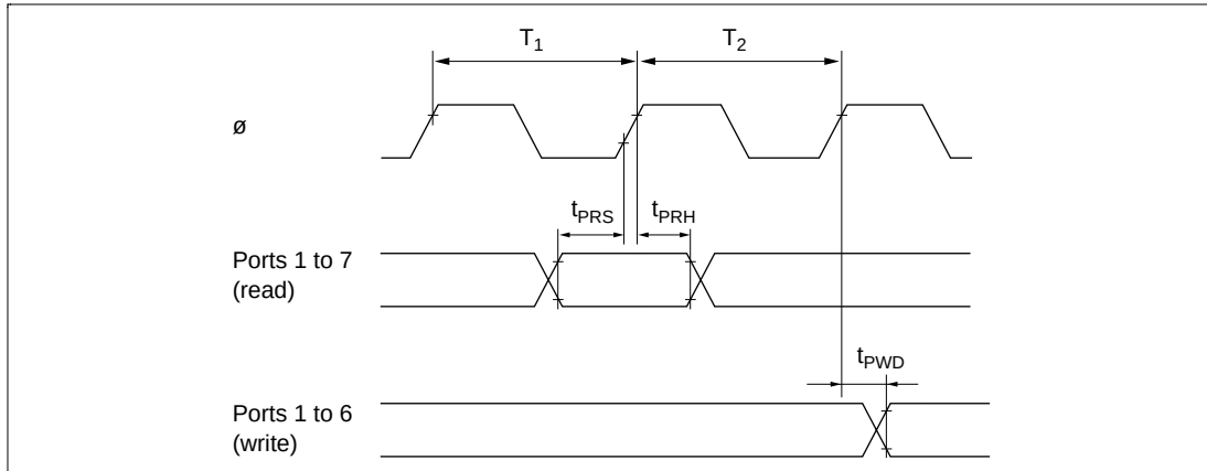
Figure 22.14 I/O Port Input/Output Timing
