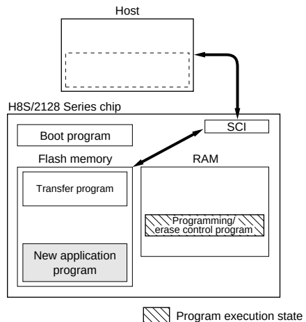
Figure 19.5 User Program Mode (Example)
