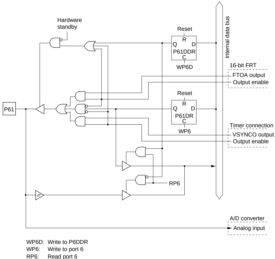
Figure C.19 Port 6 Block Diagram (Pin P61)
