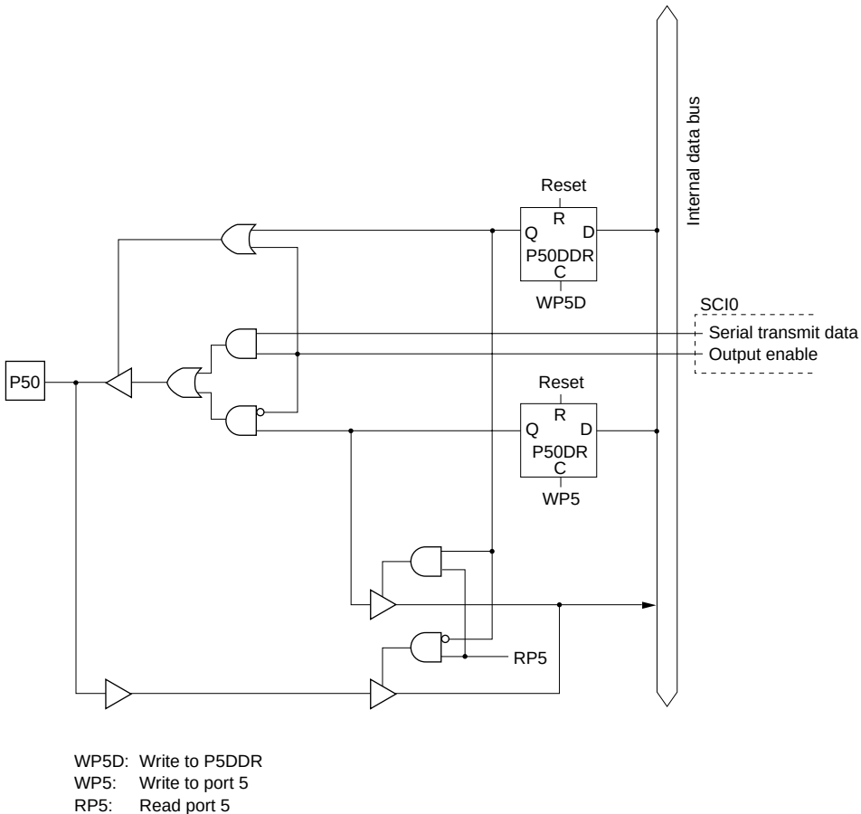
Figure C.15 Port 5 Block Diagram (Pin P50)
