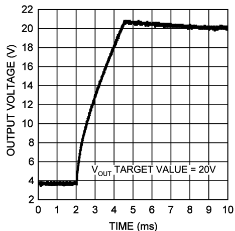
Boost Turn On Time with No Load
