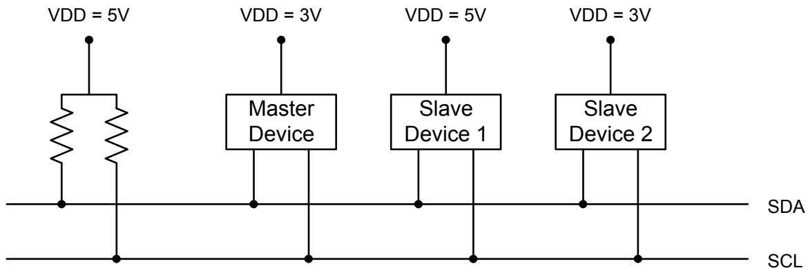
Figure 15.2. Typical SMBus Configuration
