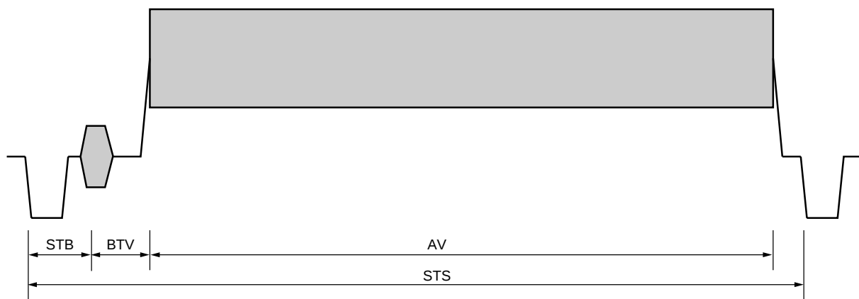
Figure 27. Horizontal Timing
