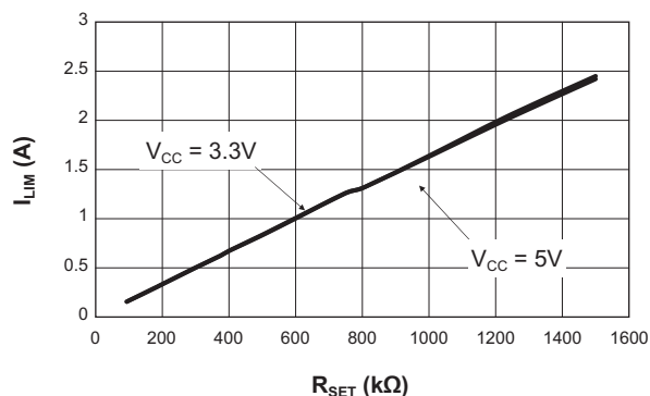
AAT4621-1 I_{LIM} vs. R_{SET} ( 25^\circ C )
