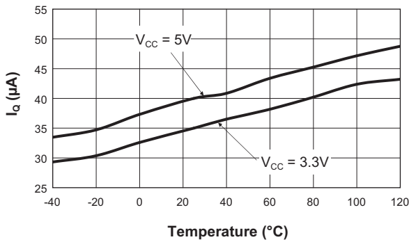
Quiescent Current I_Q vs. Temperature ( ENIU = 0V ; ENIL = V_{CC} ; or ENIL = 0V ; ENIU = V_{CC} ; V_{OUT} = Open )
