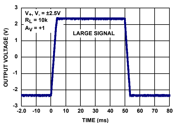
FIGURE 8. LARGE SIGNAL TRANSIENT RESPONSE
