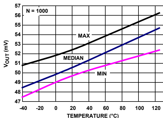
FIGURE 27. V_{OUT} LOW vs TEMPERATURE V_+, V_- = \pm 2.5V , R_L = 10
