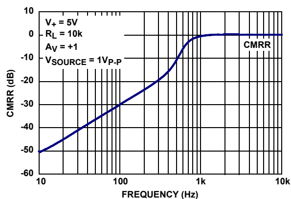
FIGURE 2. CMRR vs FREQUENCY
