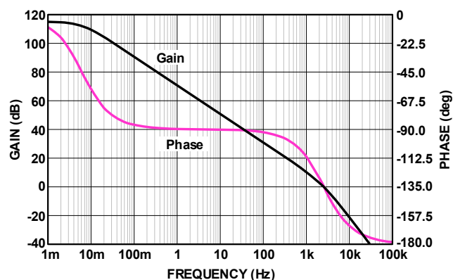
FIGURE 28. OPEN-LOOP GAIN AND PHASE vs FREQUENCY
