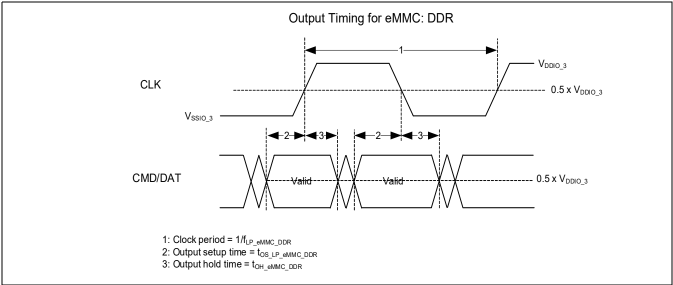
Figure 27-6 eMMC DDR output timing
