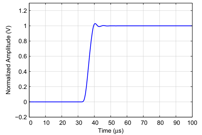
Figure 9-64. Step Response
