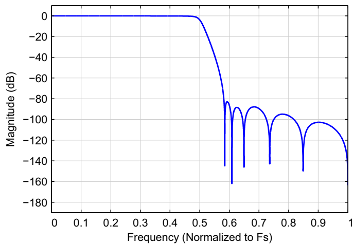
Figure 9-65. Magnitude Response
