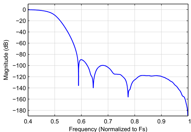
Figure 9-44. Stopband Attenuation
