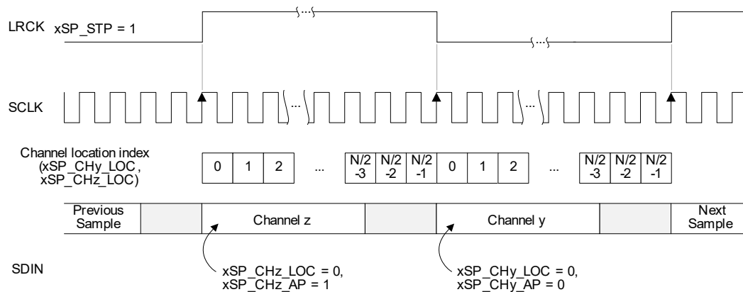
Figure 4-24. Example 50/50 Mode (ASP_STP = 1)
