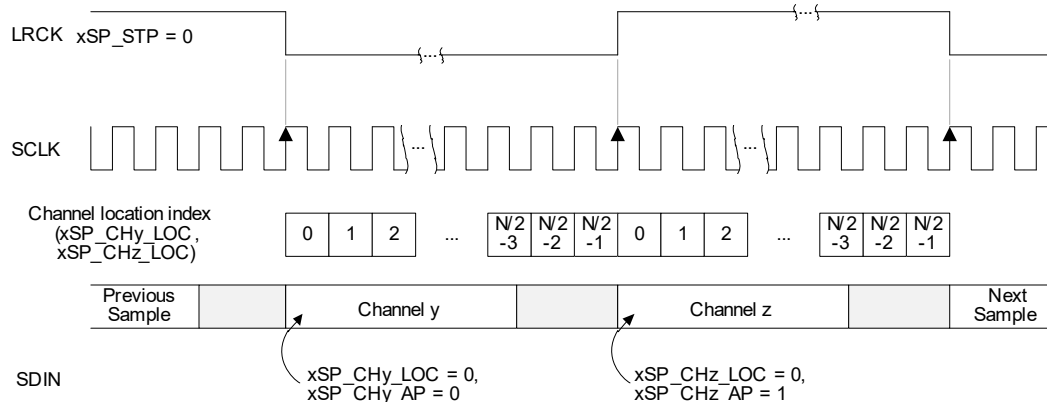
Figure 4-23. Example 50/50 Mode (ASP_STP = 0)
