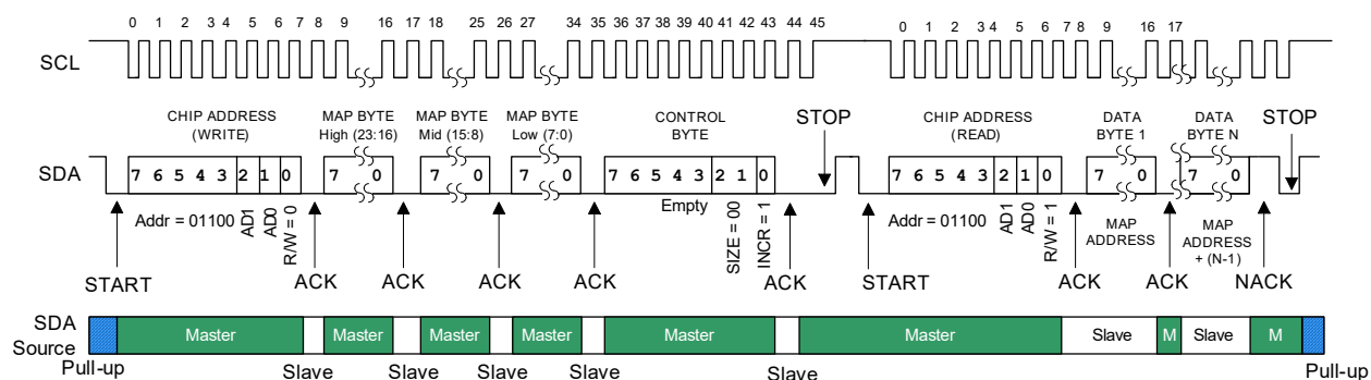
Figure 4-31. Control Port Timing, I²C Reads with Preamble and Autoincrement (8-Bit Data Access)
