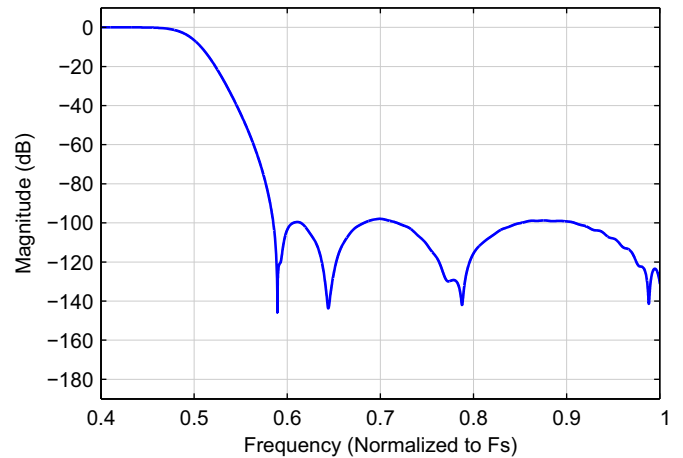
Figure 9-14. Stopband Attenuation
