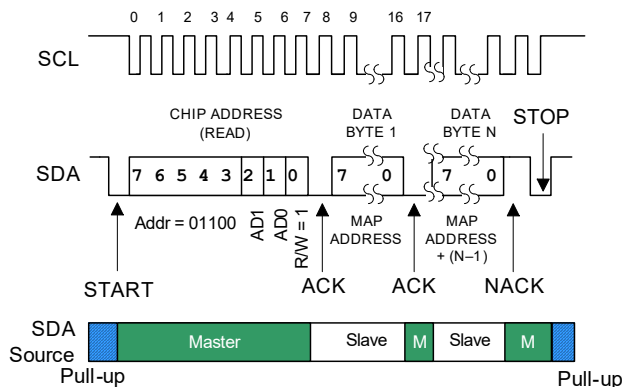
Figure 4-30. Control Port Timing, I²C Reads with Autoincrement (8-Bit Data Access)
