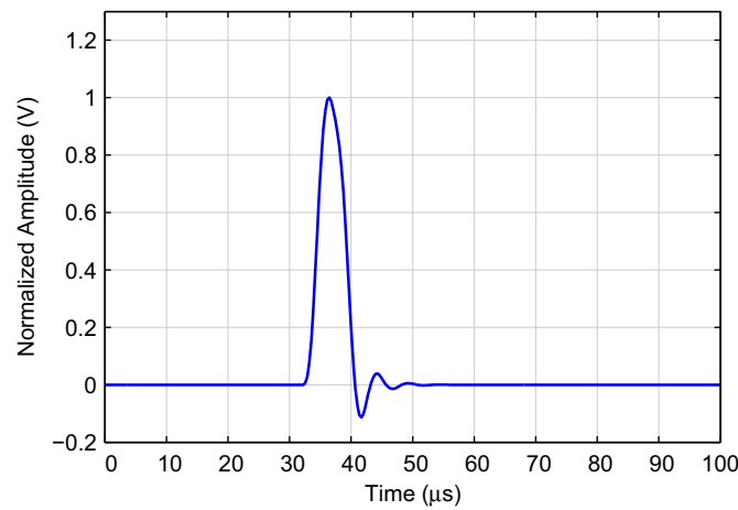
Figure 9-63. Impulse Response
