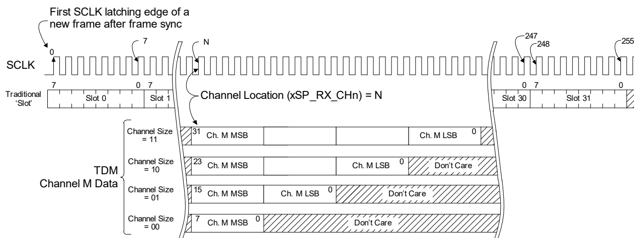
Figure 4-22. Example Channel Location and Size
