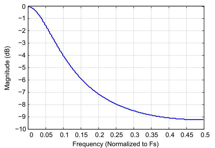
Figure 9-71. Deemphasis
