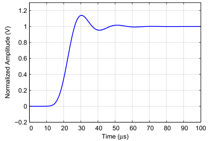
Figure 9-69. Step Response
