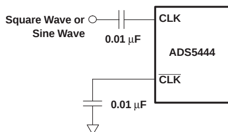
Figure 37. Single-Ended Clock
