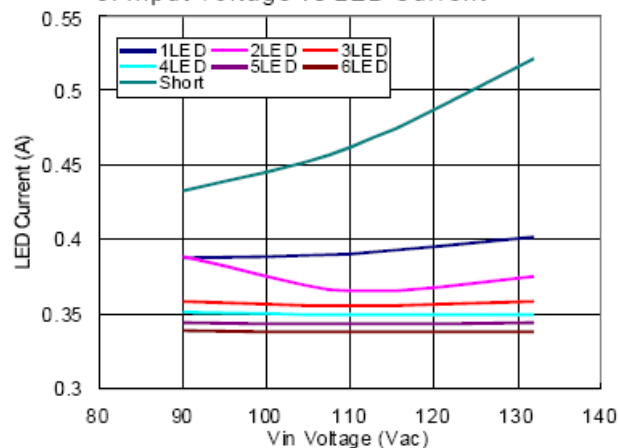
8. Input Voltage vs LED Current
