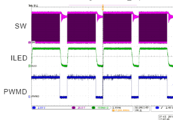
12. PWM Dimming use PWM_D pin
