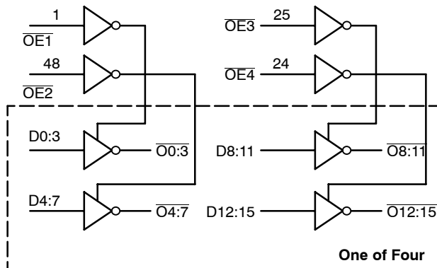
Figure 2. Logic Diagram
