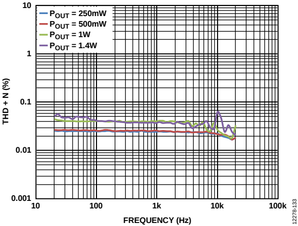
Figure 33. Current Sense THD + N vs. Frequency, V_{BAT} = 3.6\text{ V} , R_L = 4\ \Omega and 15\ \mu\text{H}
