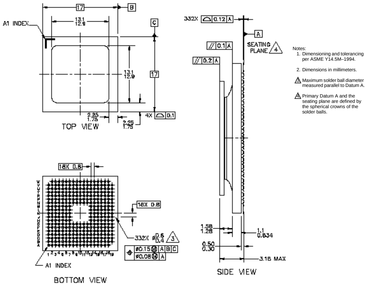
CASE 1473-01
