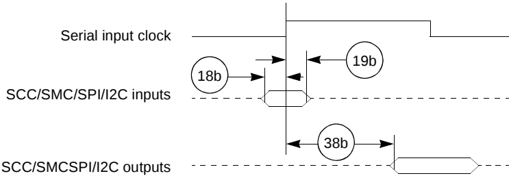
Figure 2-21. SCC/SMC/SPI/I 2 C External Clock Diagram
