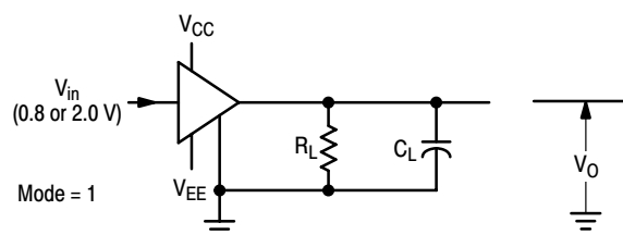
Figure 2. Single-Ended Output Test
