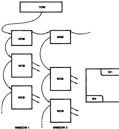
Figure 6. Window Data Structure
