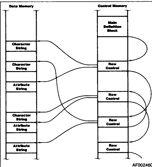
Figure 4. Am8052 Linked-List Structure
