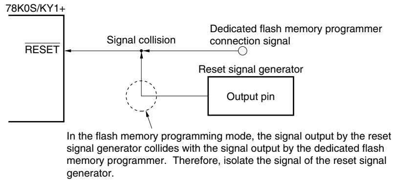
Figure 16-6. Signal Collision (RESET Pin)
