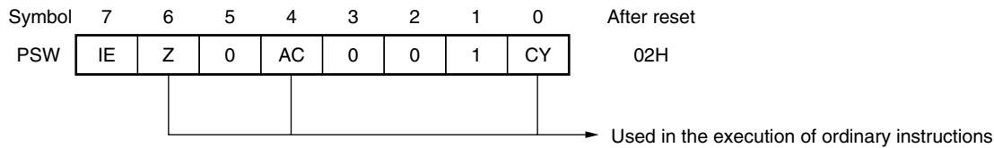
Figure 10-5. Program Status Word (PSW) Configuration
