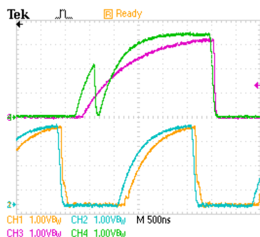
Fig 10. Fast rising SDA_xx 'input' side
