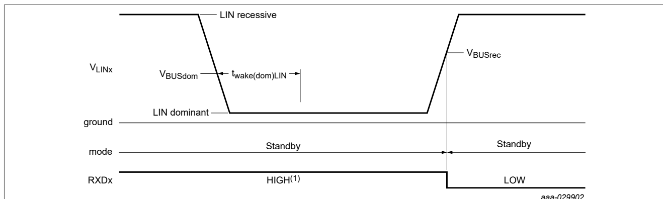
Figure 5. Principle of remote wake-up via LIN bus in Standby mode
