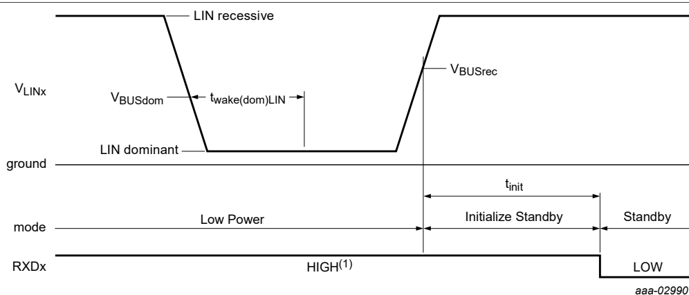
Figure 4. Principle of remote wake-up via LIN bus in Low Power mode
