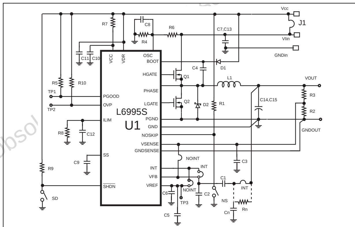
Figure 16. Schematic Diagram
