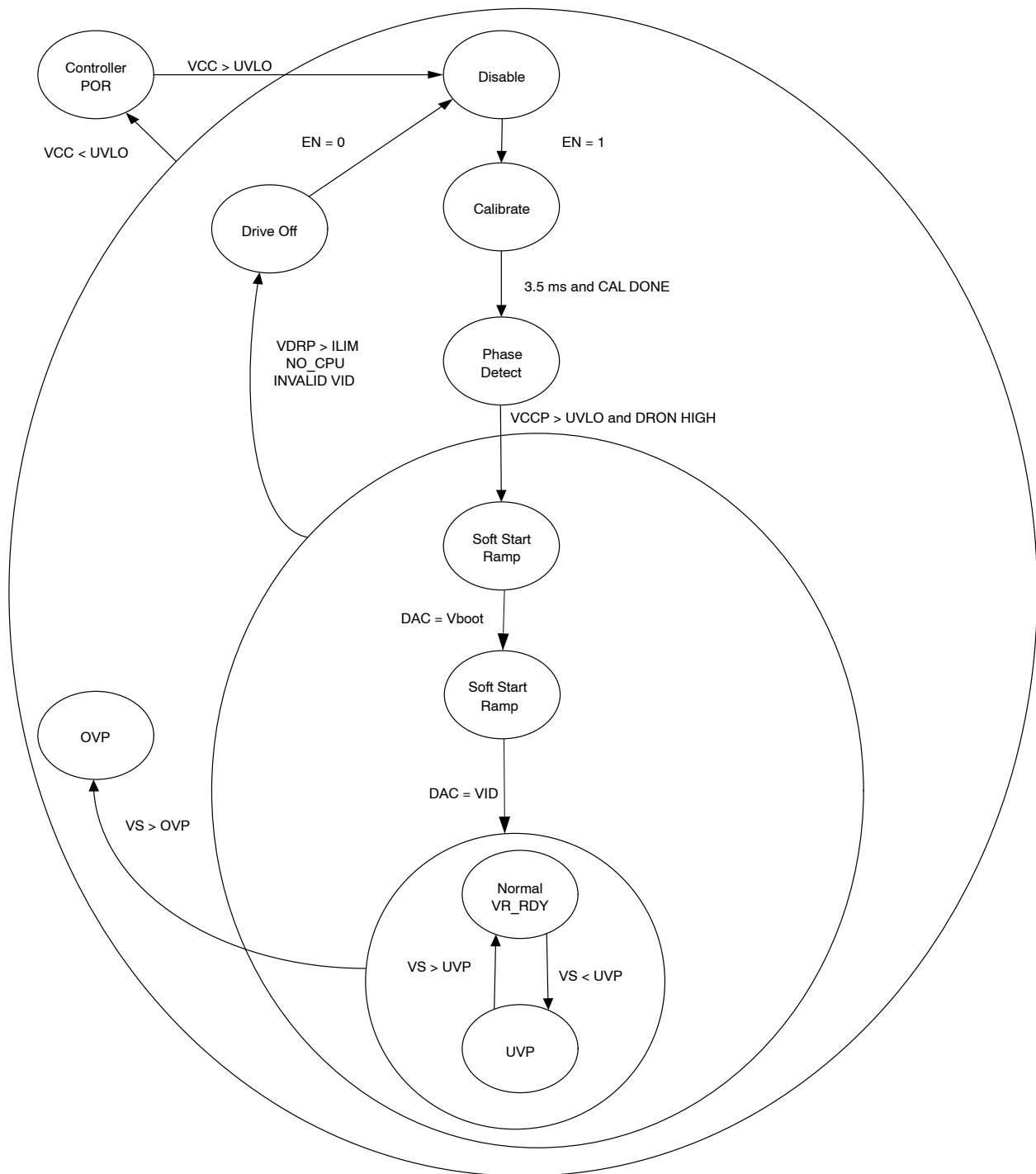
Figure 11. State Diagram
