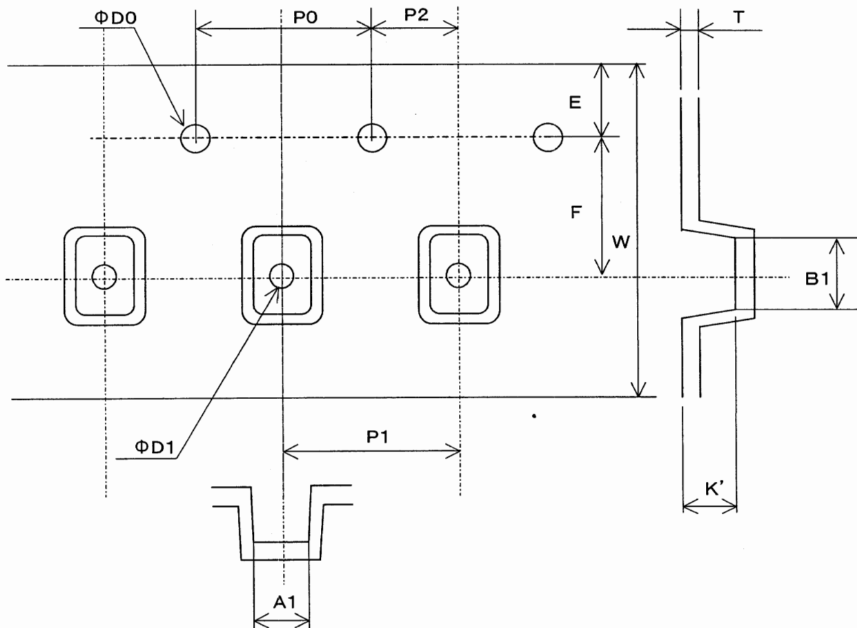
Figure8. Taping dimensions
