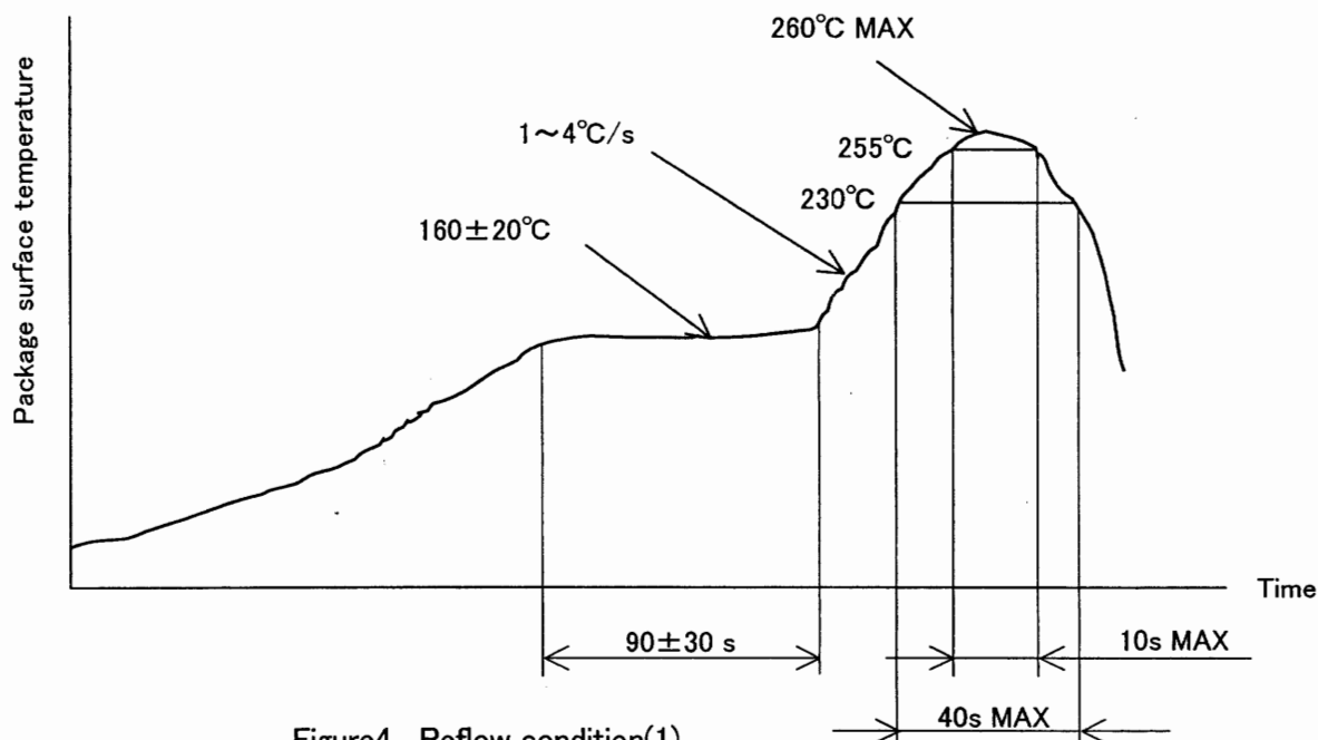
Figure4. Reflow condition(1)
