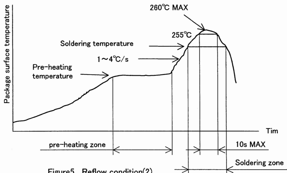
Figure5. Reflow condition(2)
