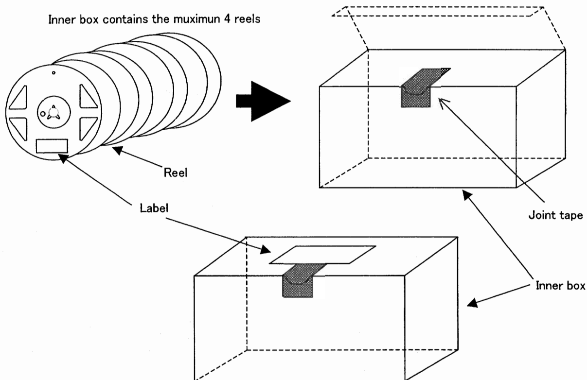
Figure11. Packing methods
