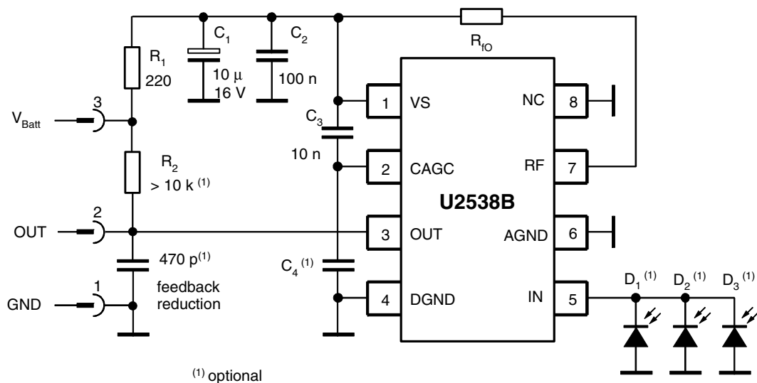
Figure 6-2. Application Circuit
