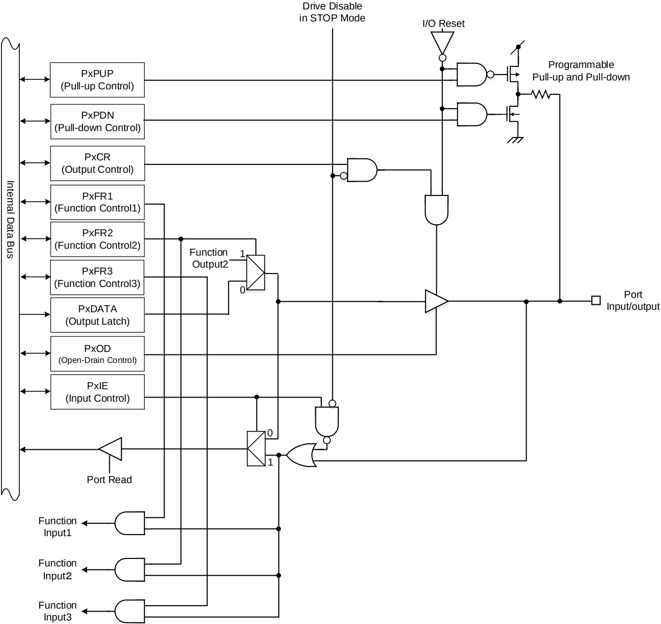
Figure 8.15 Port Type T15
