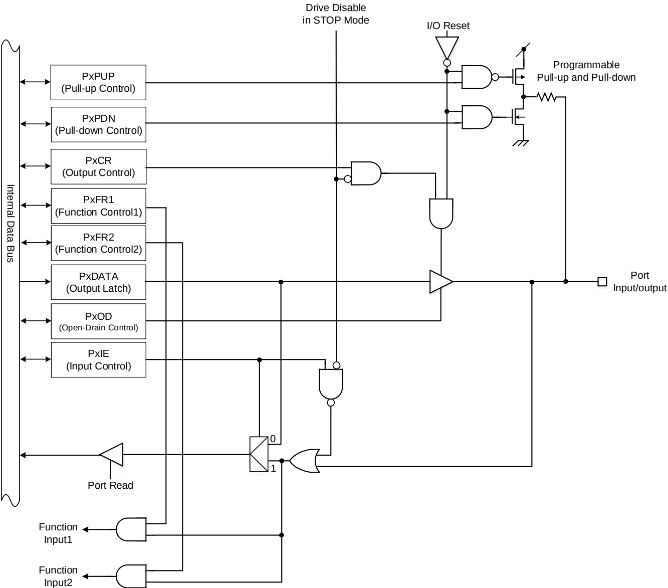
Figure 8.11 Port Type T11
