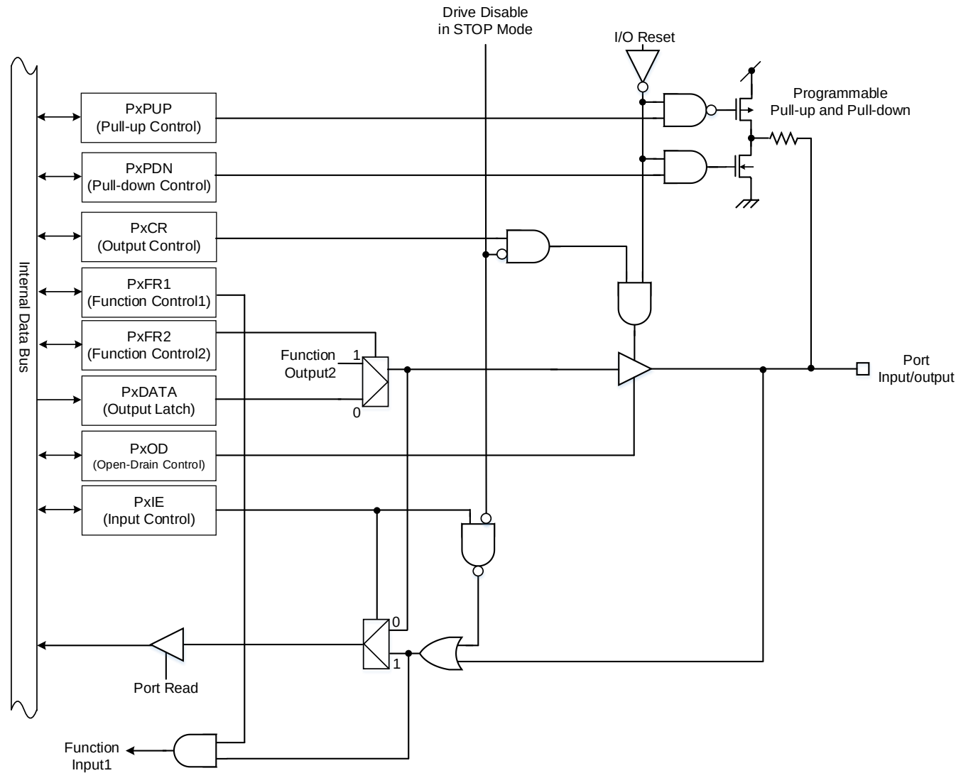
Figure 8.10 Port Type T10
