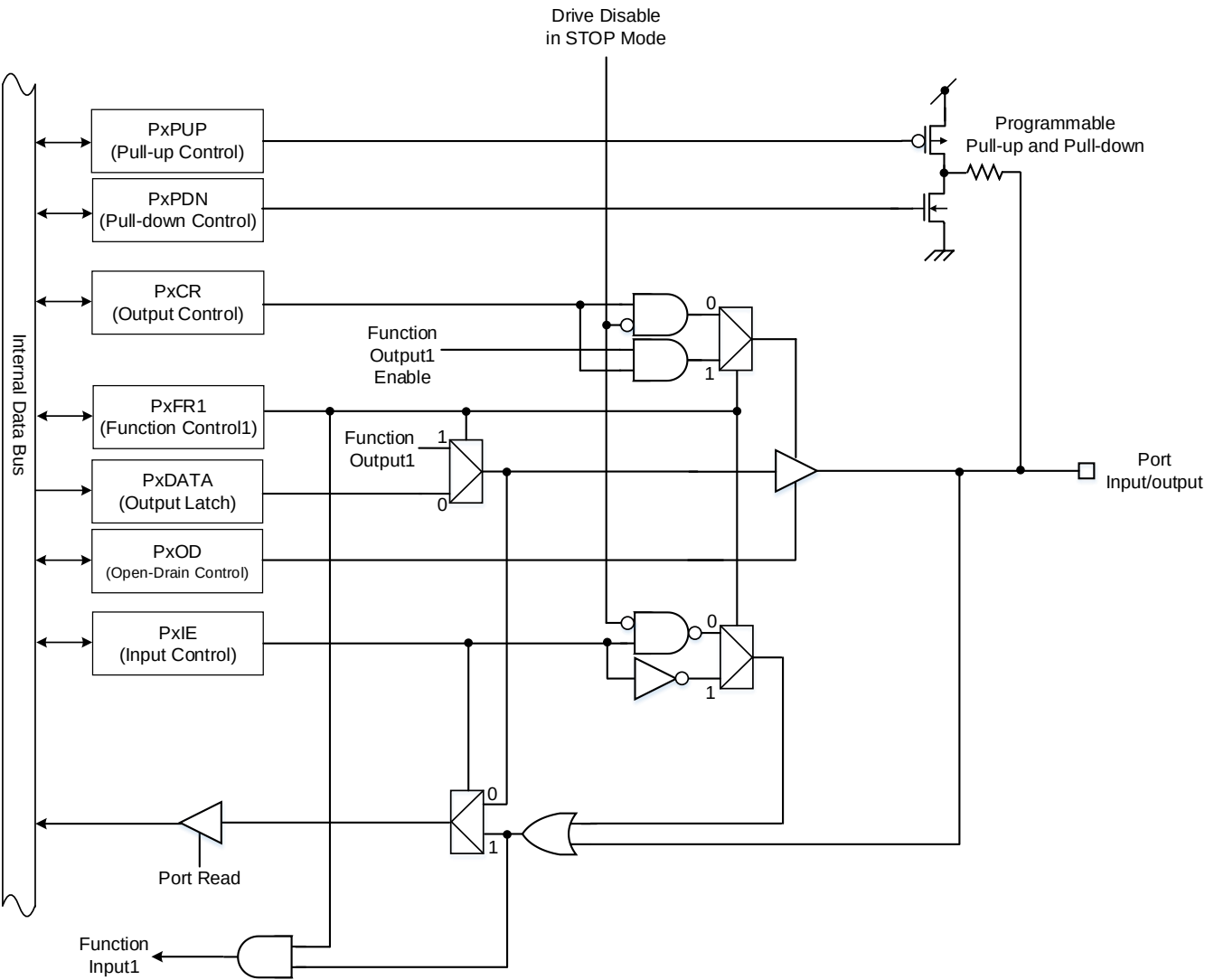
Figure 8.6 Port Type T6
