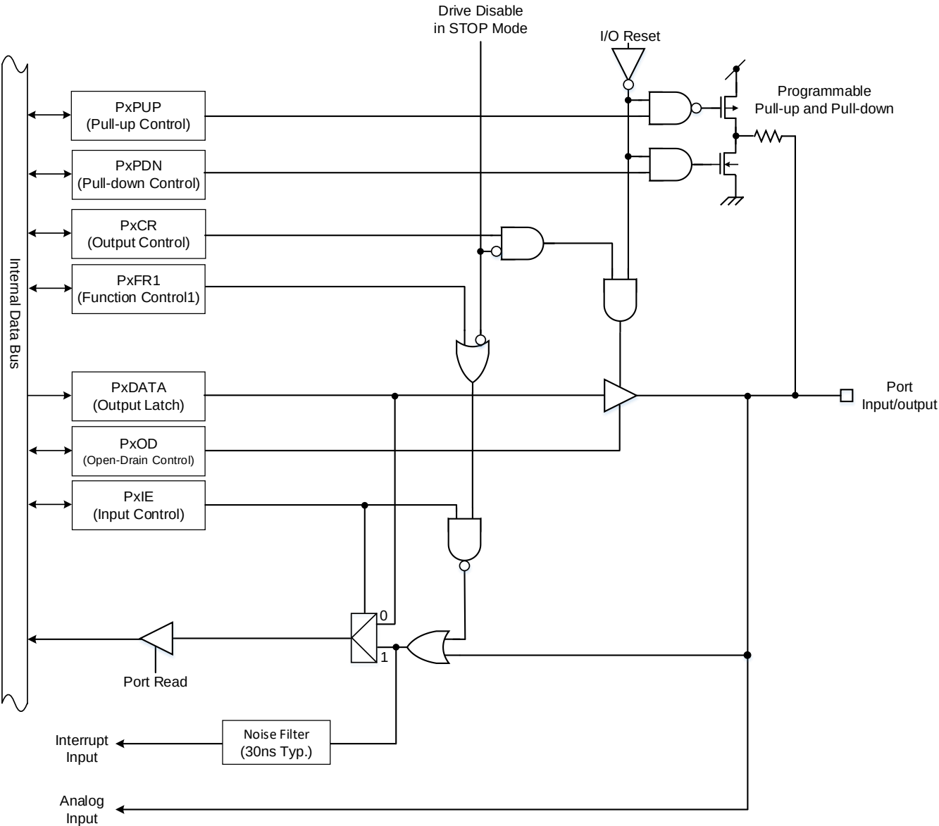
Figure 8.17 Port Type T17
