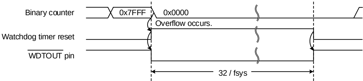
Figure 18.3 Timing of Watchdog Timer Reset Generation
