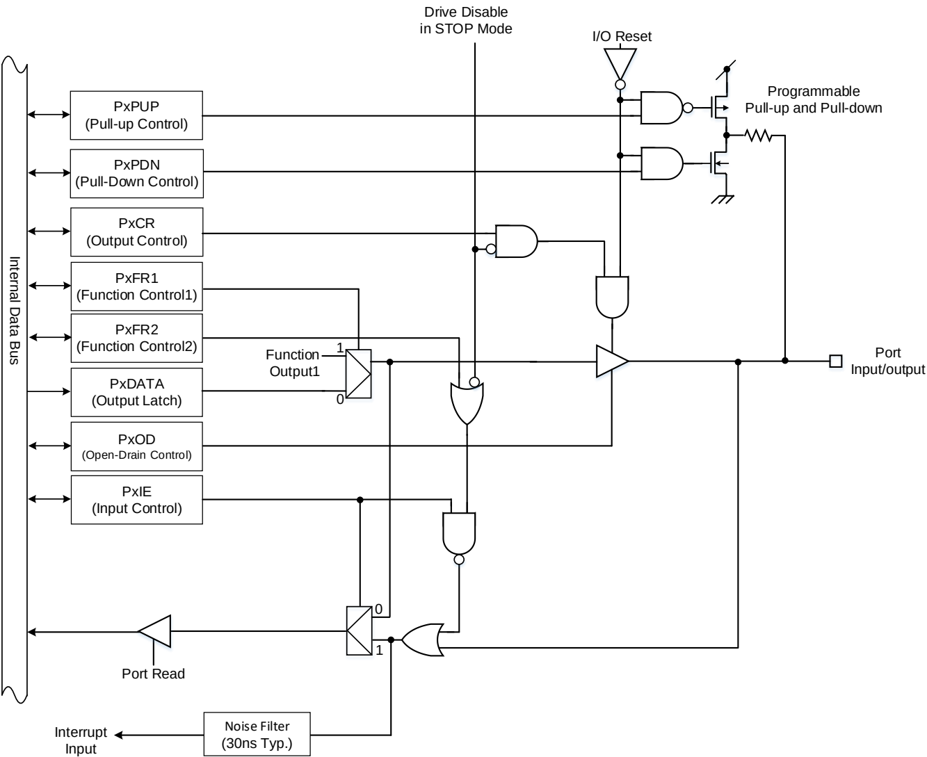
Figure 8.14 Port Type T14
