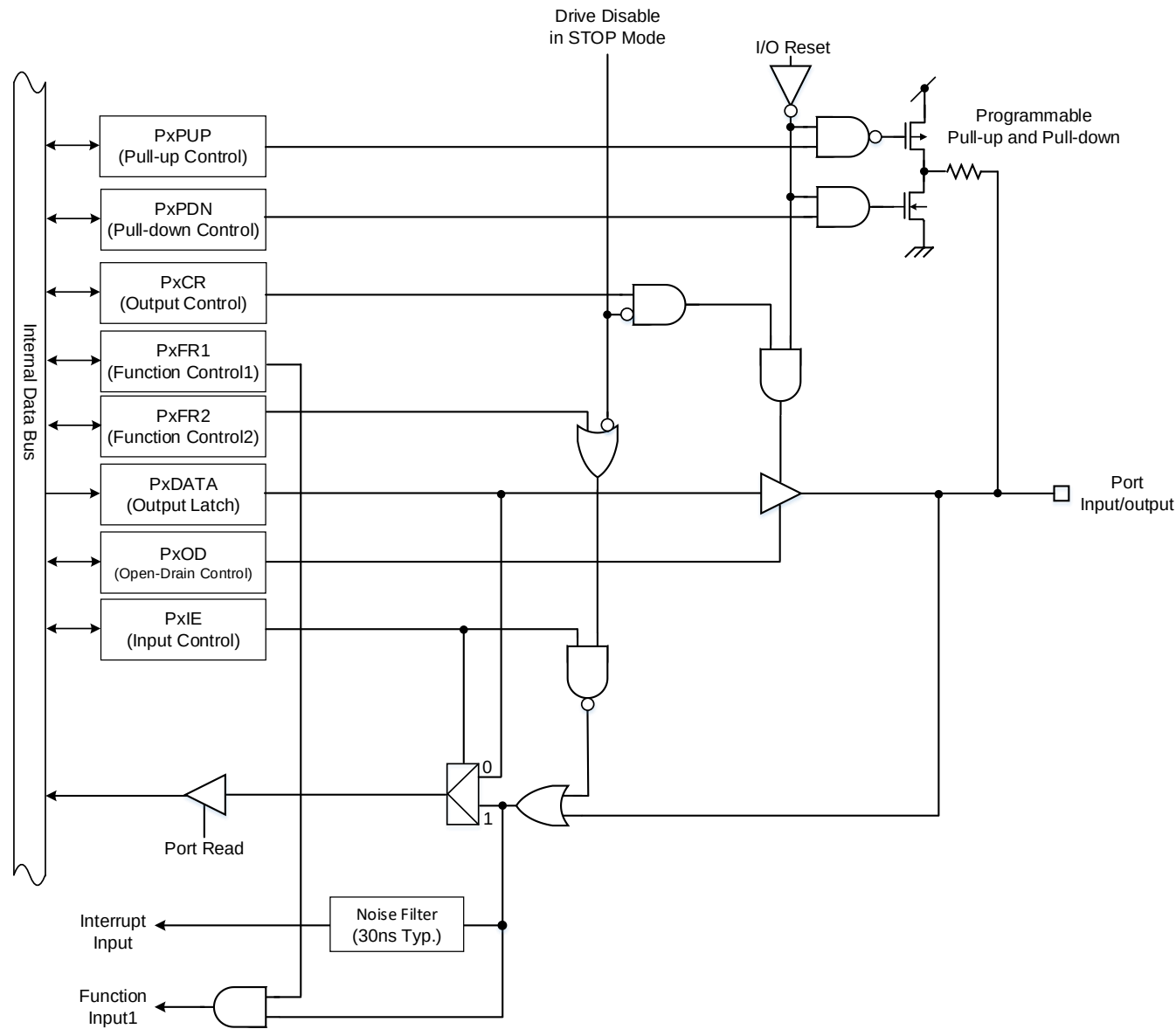
Figure 8.12 Port Type T12
