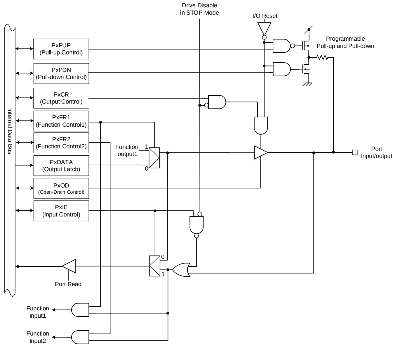
Figure 8.9 Port Type T9
