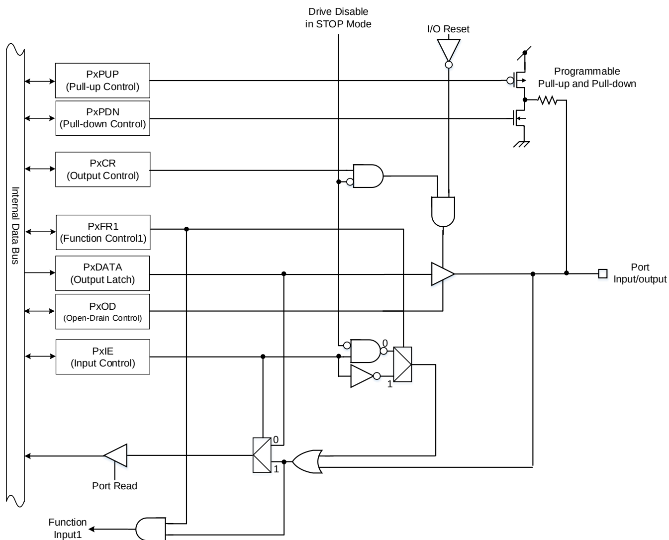
Figure 8.7 Port Type T7
