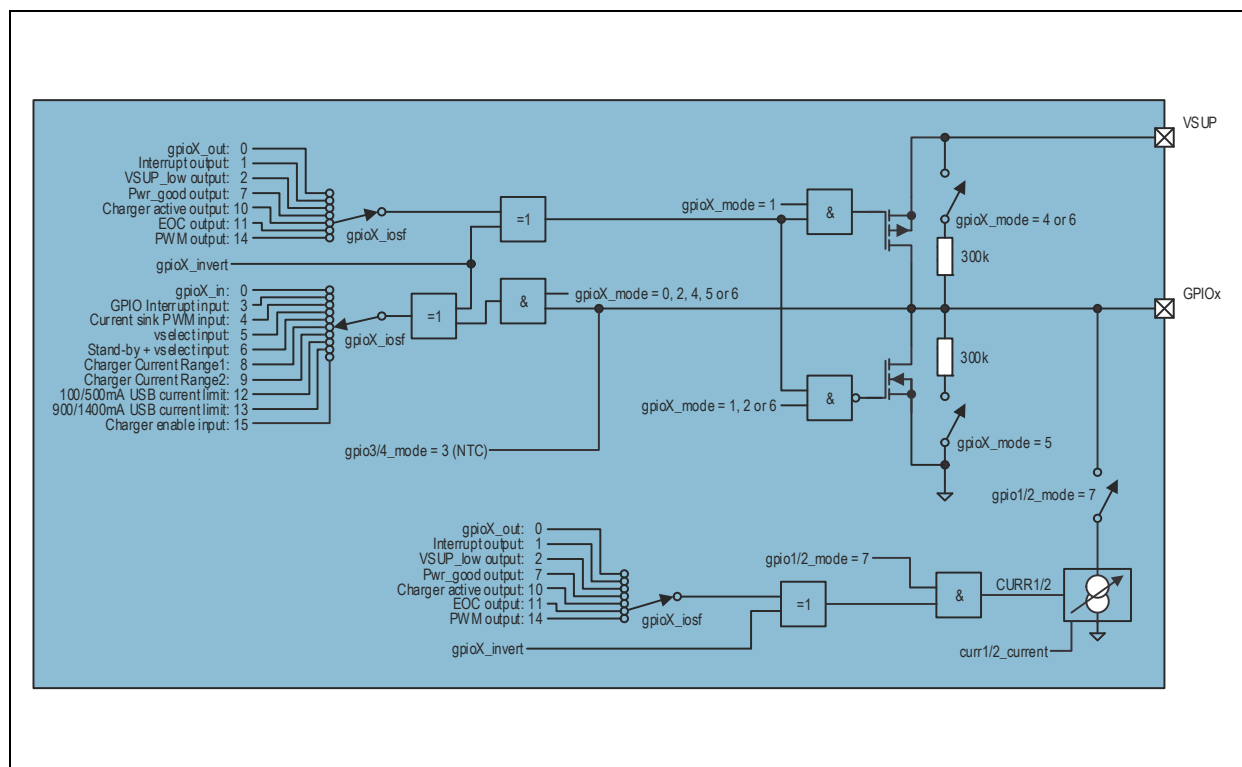
Figure 48: GPIO Block Diagram
