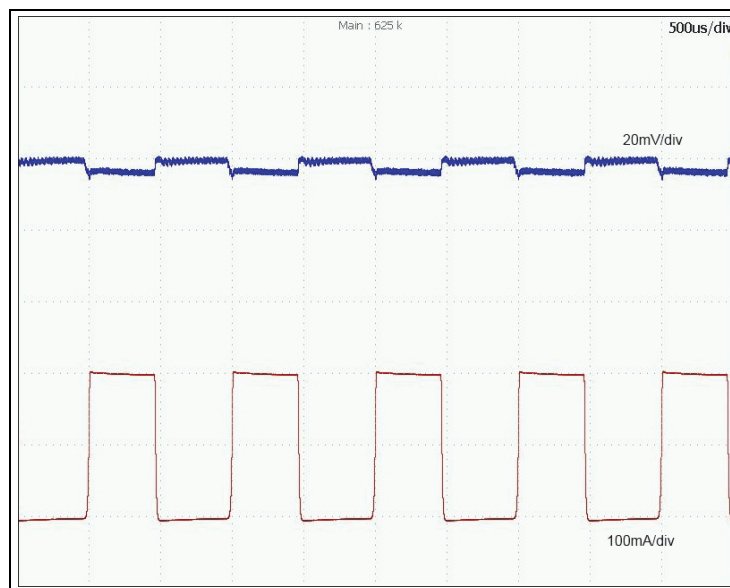
Figure 28: LDO Load Transient Response 2/2
