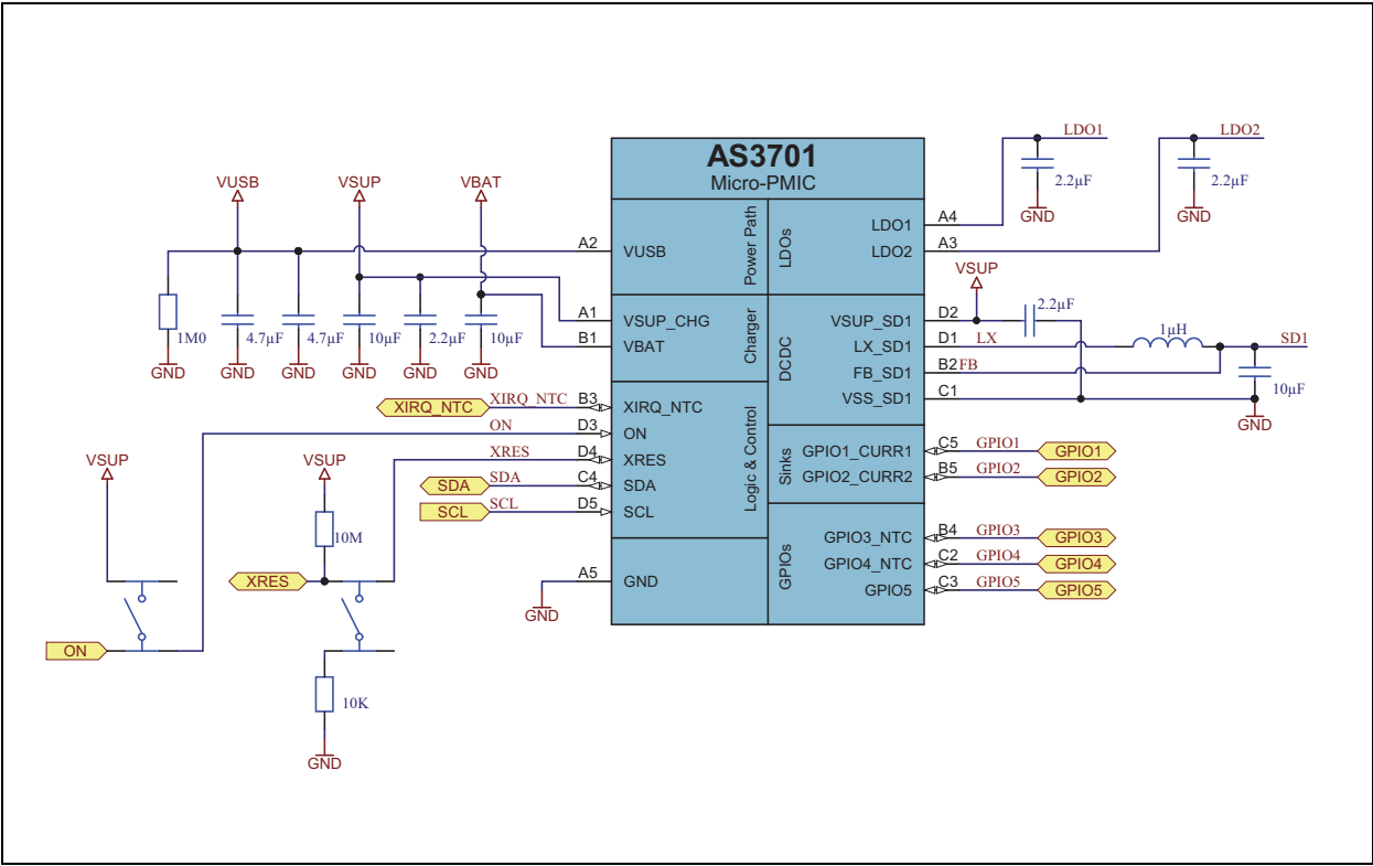
Figure 114: Application Schematic
