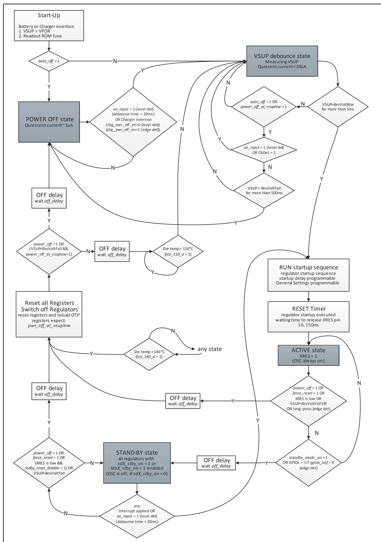
Figure 40: Start-Up Flowchart
