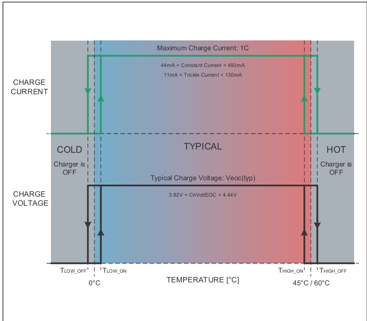
Figure 36: High/Low Temperature Supervision
