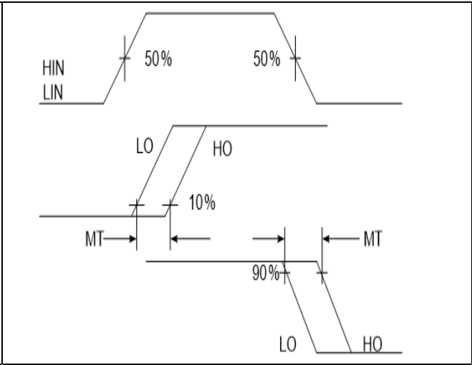
Figure 11 Delay Matching Waveform Definitions
