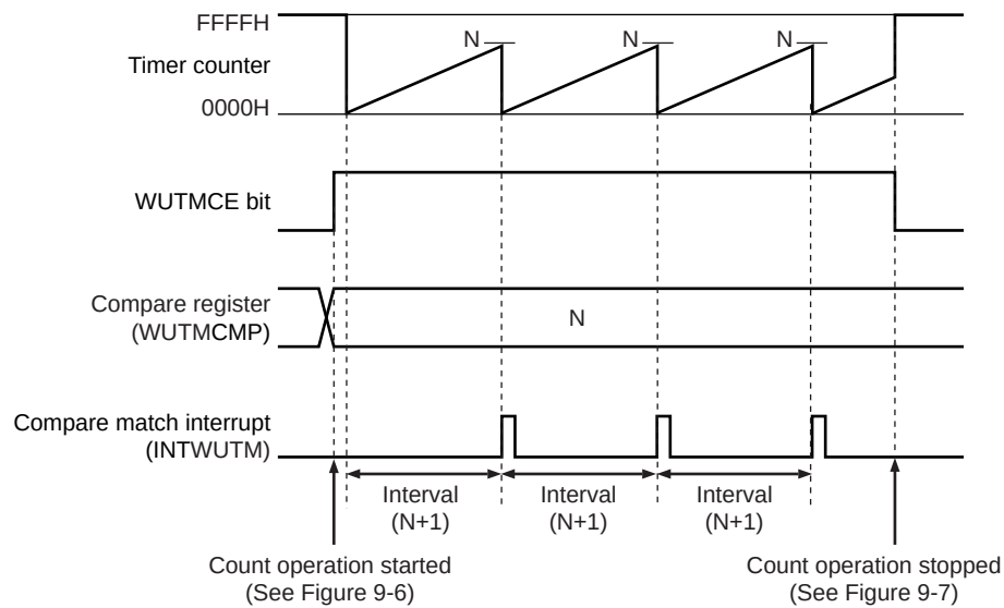
Figure 9-8. Operation Timing of Interval Timer Mode
