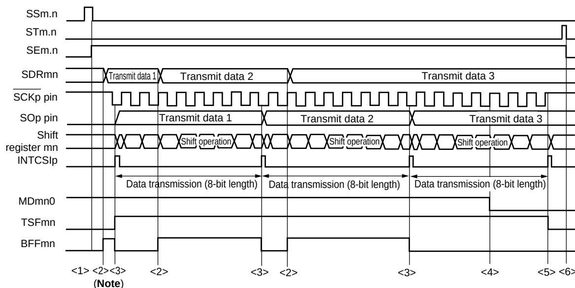
Figure 13-64. Timing Chart of Slave Transmission (in Continuous Transmission Mode)
