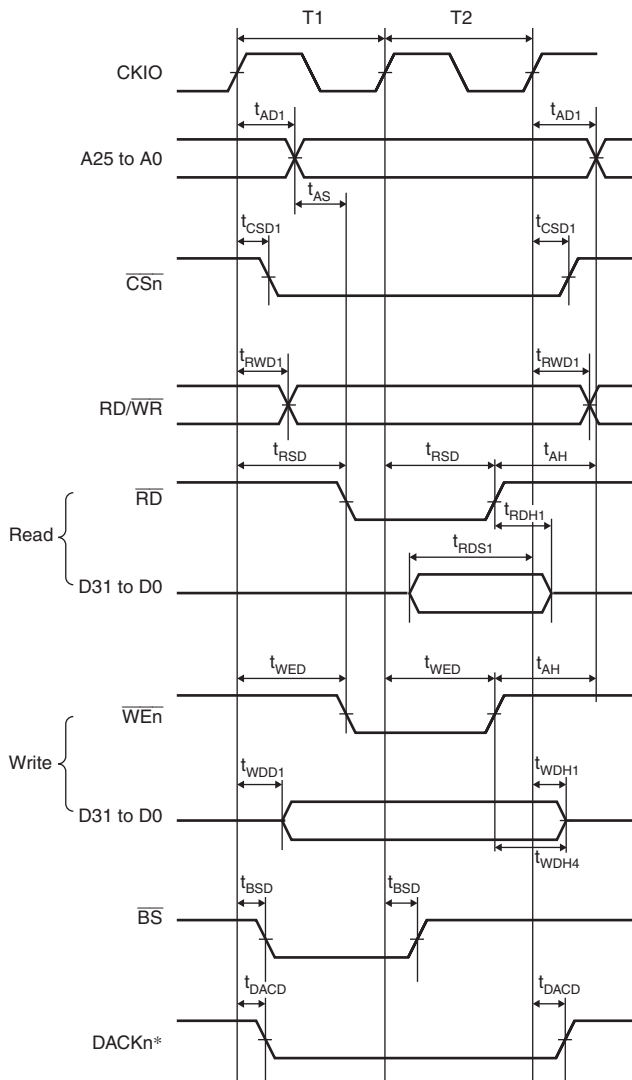
Figure 25.17 Basic Bus Cycle (No Wait)
