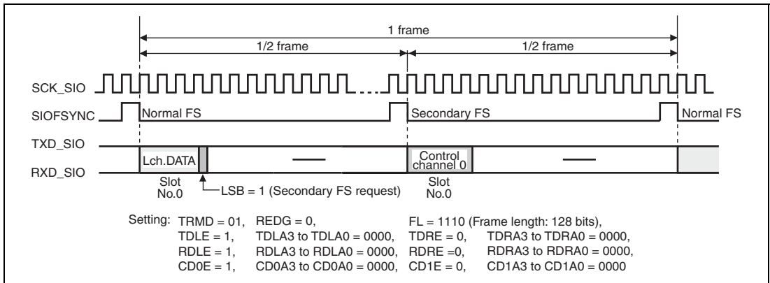
Figure 17.8 Control Data Interface (Secondary FS)
