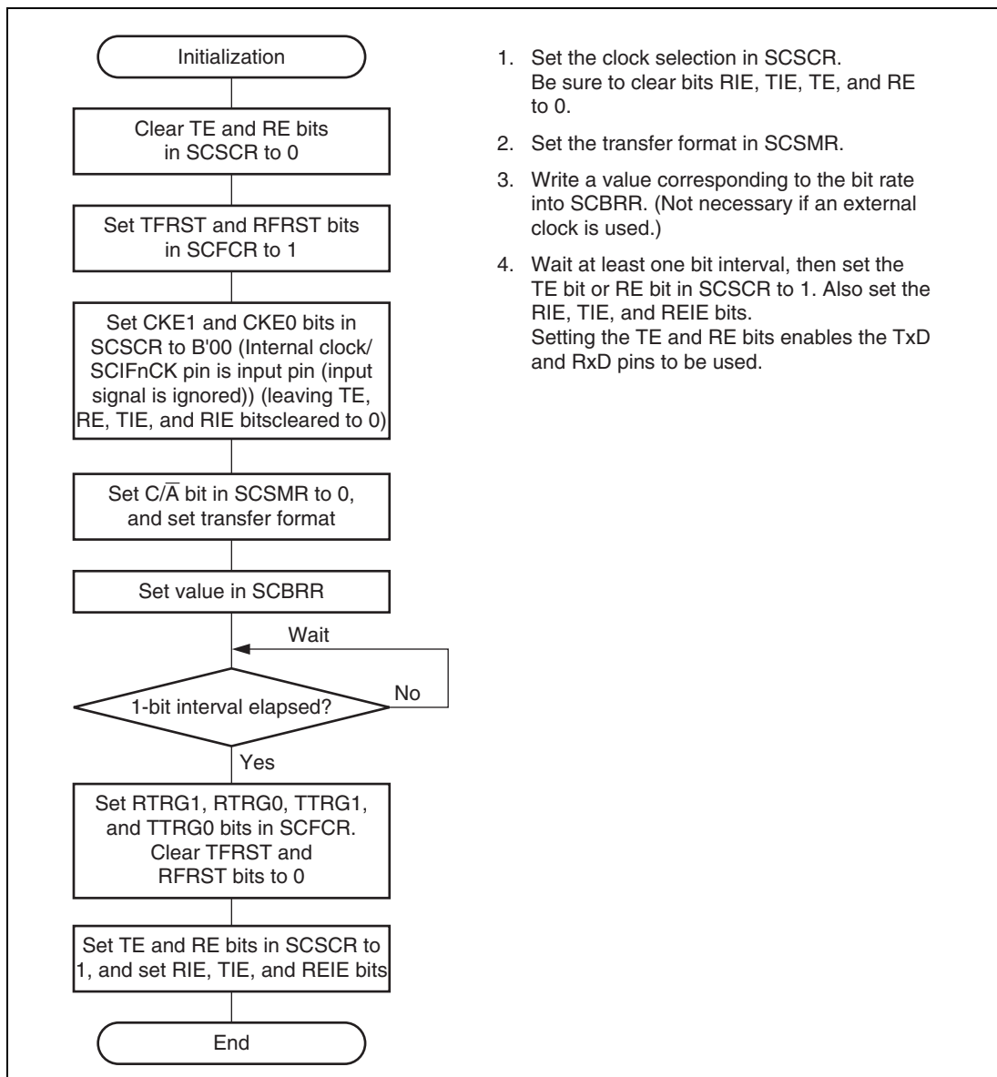
Figure 16.3 Sample SCIF Initialization Flowchart
