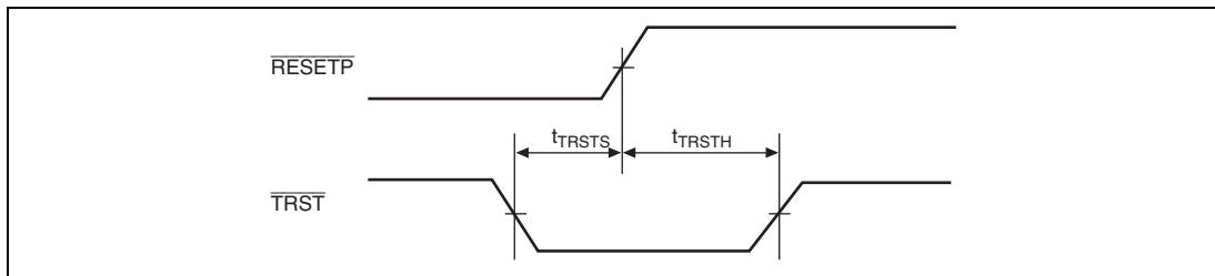
Figure 25.70 \overline{\text{TRST}} Input Timing (Reset Hold)
