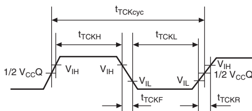
Figure 25.69 TCK Input Timing
