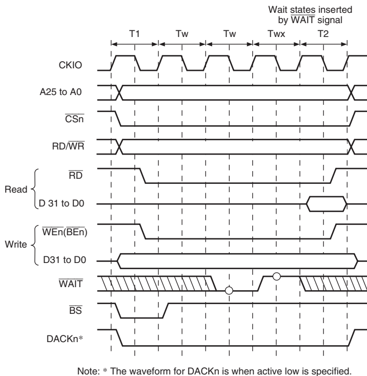
Figure 12.10 Wait State Timing for Normal Space Access (Wait State Insertion by \overline{\text{WAIT}} Signal)
