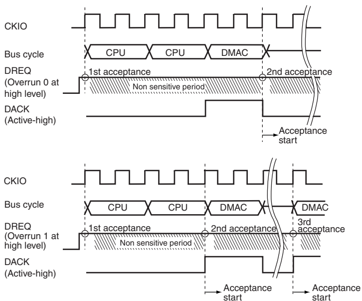
Figure 13.15 Example of DREQ Input Detection in Burst Mode Level Detection
