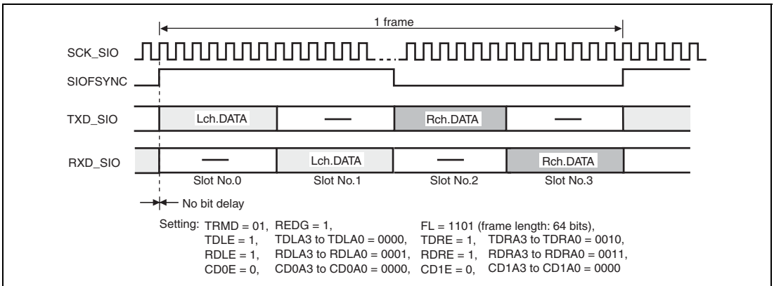
Figure 17.17 Transmission and Reception Timings (16-Bit Stereo Data (2))
