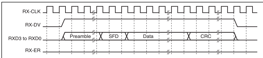
Figure 18.7 (4) MII Frame Receive Timing (Normal Reception)
