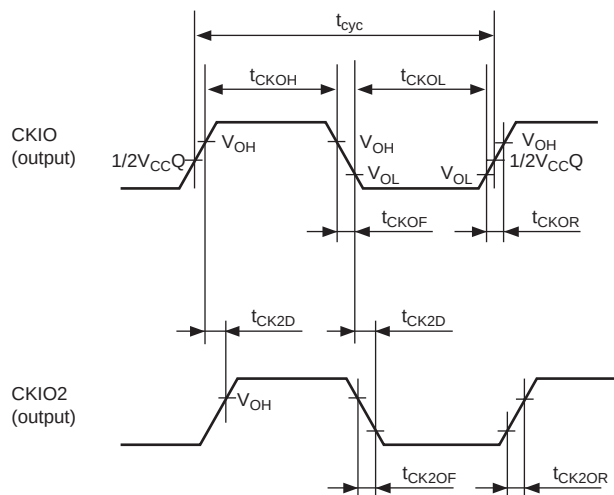
Figure 25.4 CKIO Clock Output Timing
