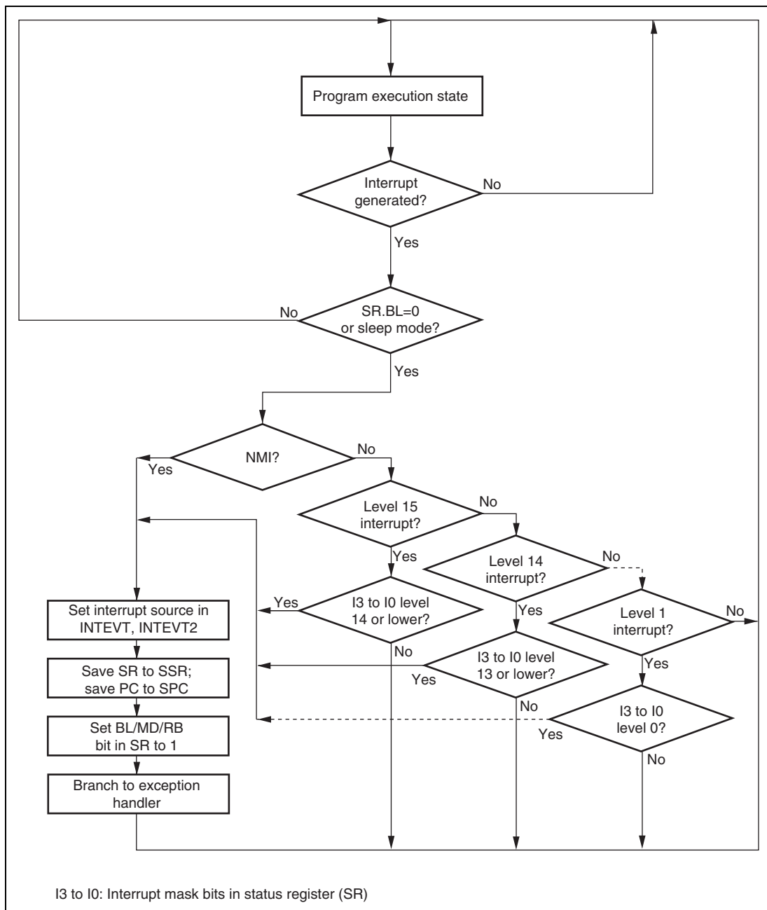
Figure 8.3 Interrupt Operation Flowchart
