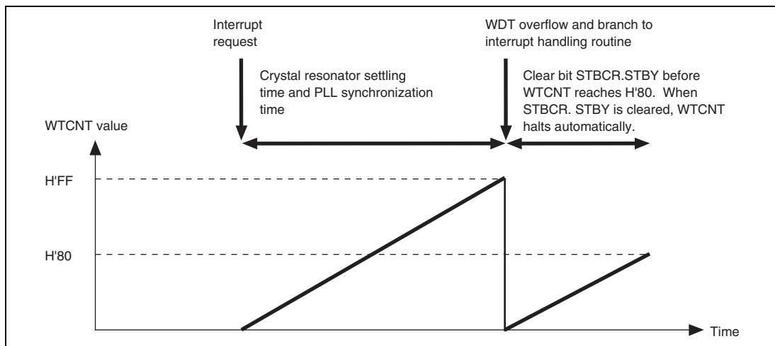
Figure 10.1 Canceling Standby Mode with STBCR.STBY
