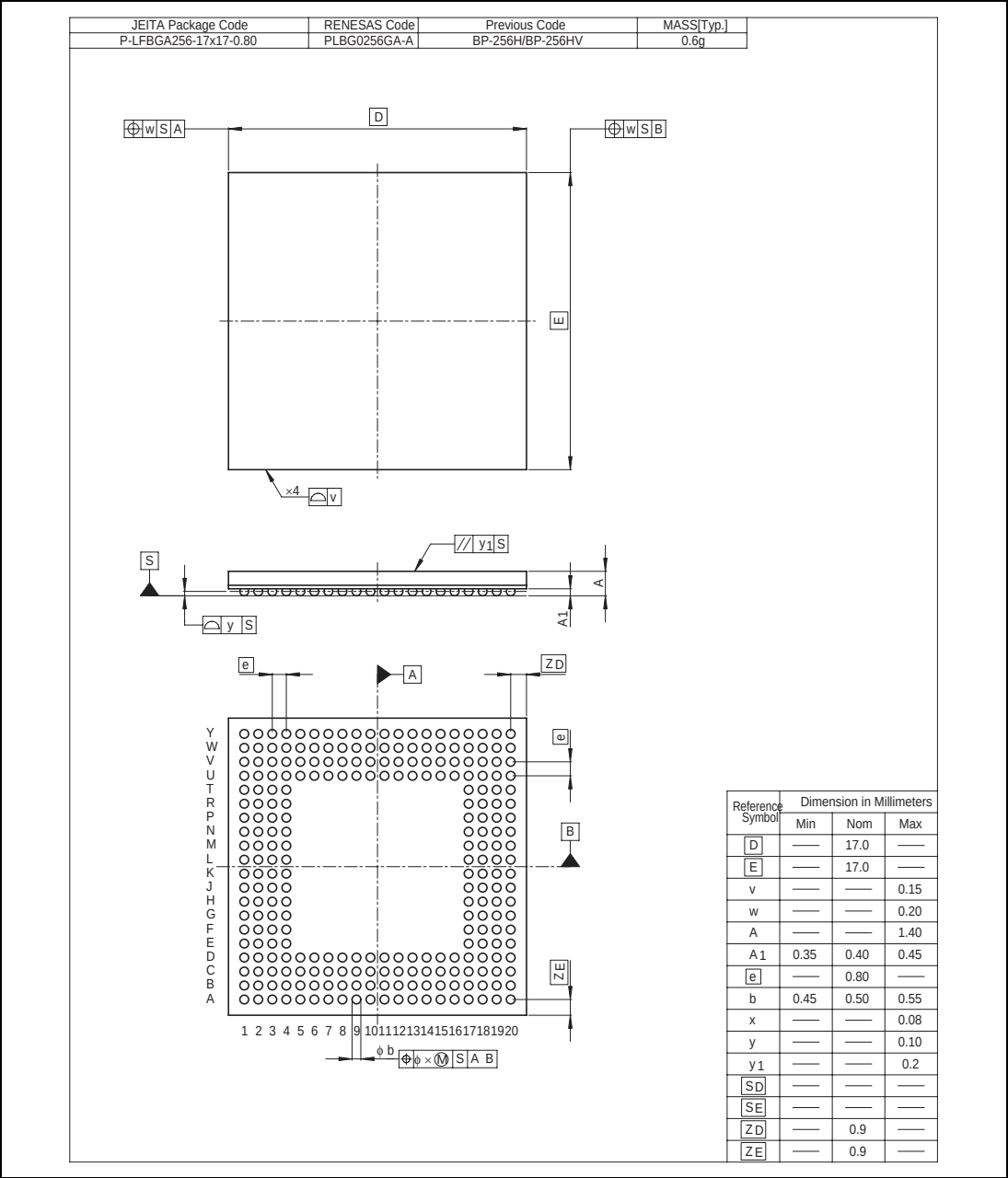
Figure B.2 Package Dimensions (P-LFBGA1717-256 (BP-256H/HV))
