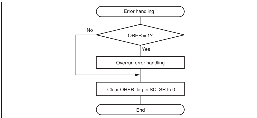
Figure 16.16 Sample Serial Reception Flowchart
