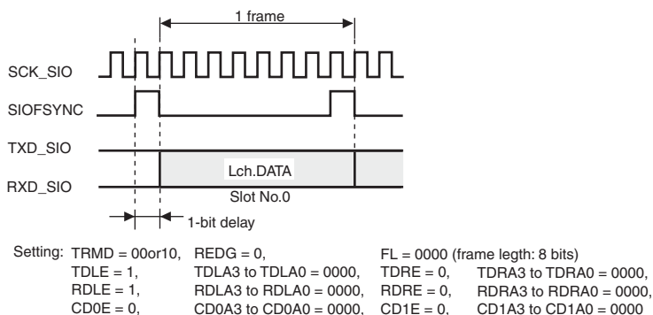
Figure 17.13 Transmission and Reception Timings (8-Bit Monaural Data (1))
