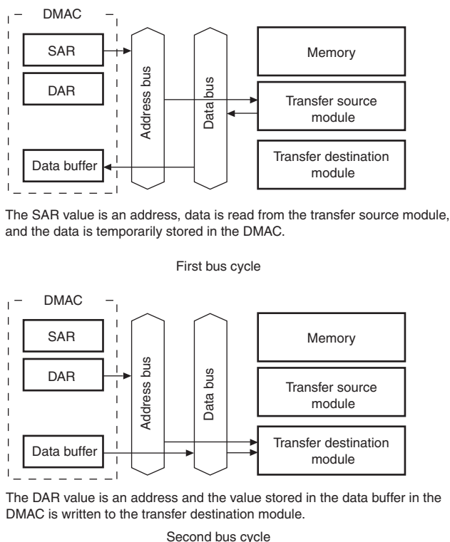
Figure 13.5 Data Flow in Dual Address Mode
