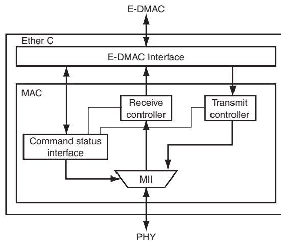
Figure 18.1 (2) Configuration of EtherC (SH7713)
