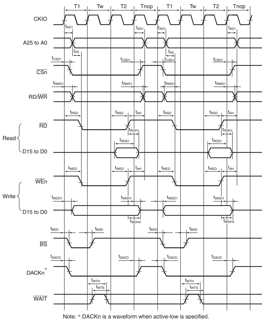
Figure 25.20 Basic Bus Cycle (One Software Wait, External Wait Enabled (WM bit = 0), No Idle Cycle Setting)
