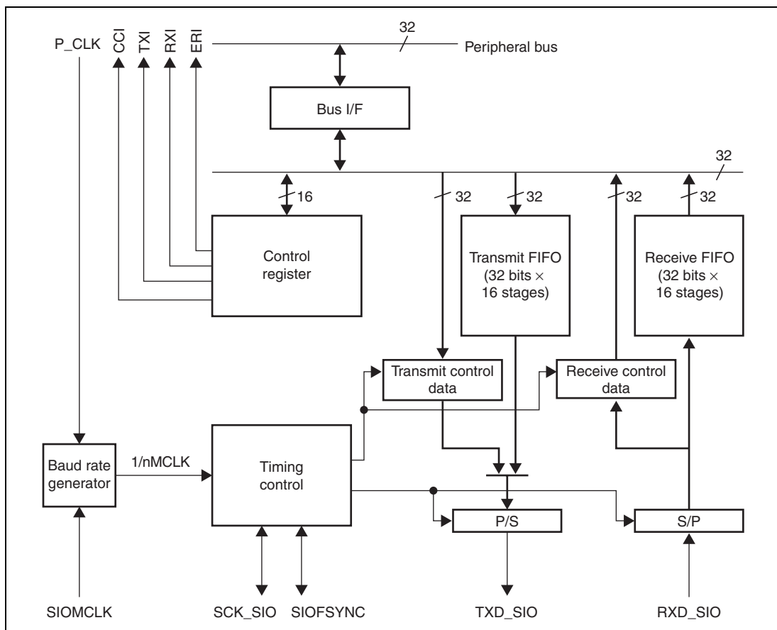
Figure 17.1 Block Diagram of SIOF
