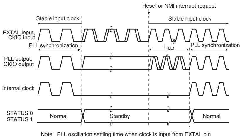
Figure 25.9 PLL Synchronization Settling Time by Reset or NMI
