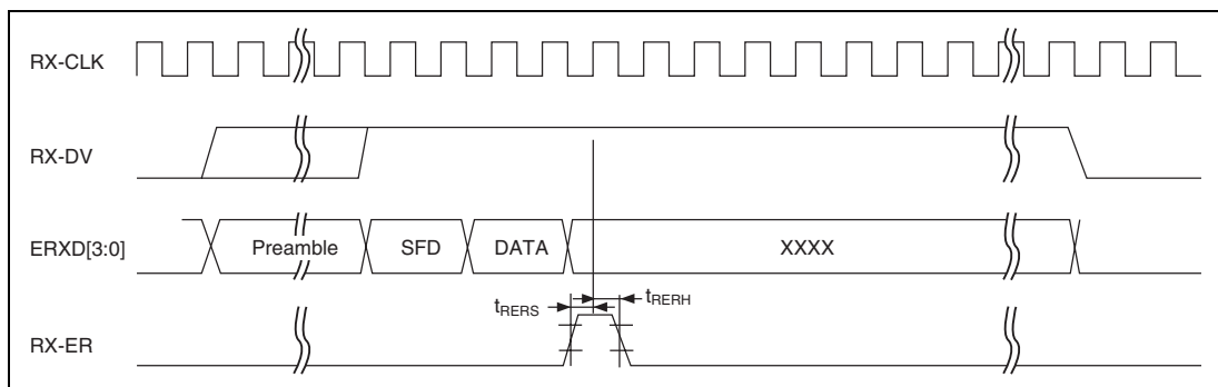
Figure 25.62 MII Receive Timing (Case of Error)
