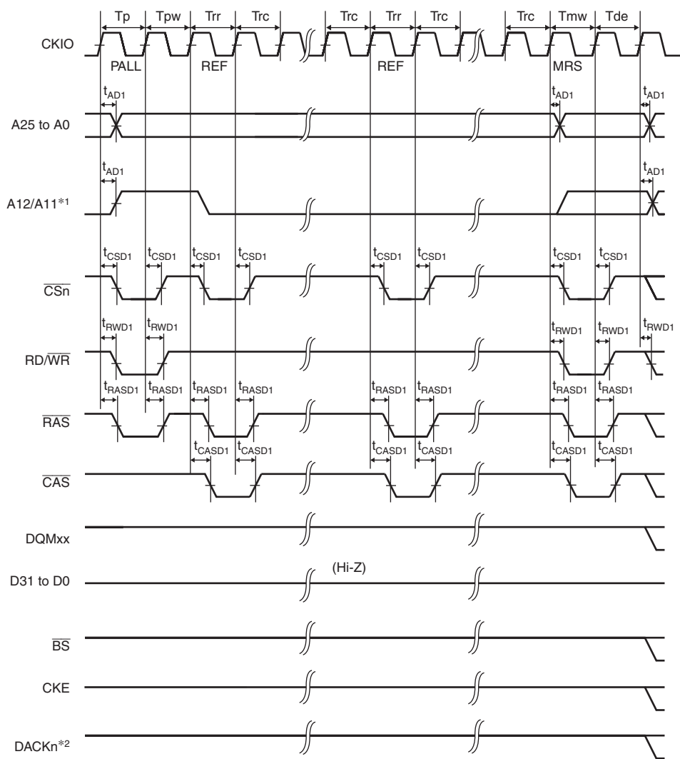
Figure 25.38 Synchronous DRAM Mode Register Write Timing (WTRP = 1 Cycle)
