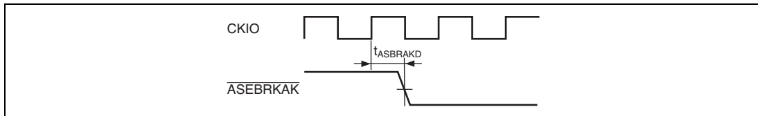
Figure 25.73 \overline{\text{ASEBRKAK}} Delay Time
