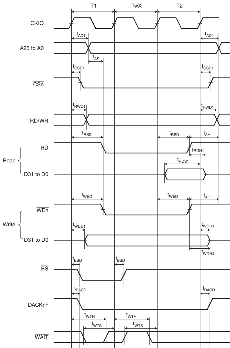
Figure 25.19 Basic Bus Cycle (One External Wait)
