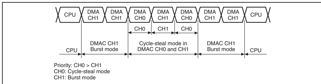
Figure 13.11 Bus State when Multiple Channels are Operating
