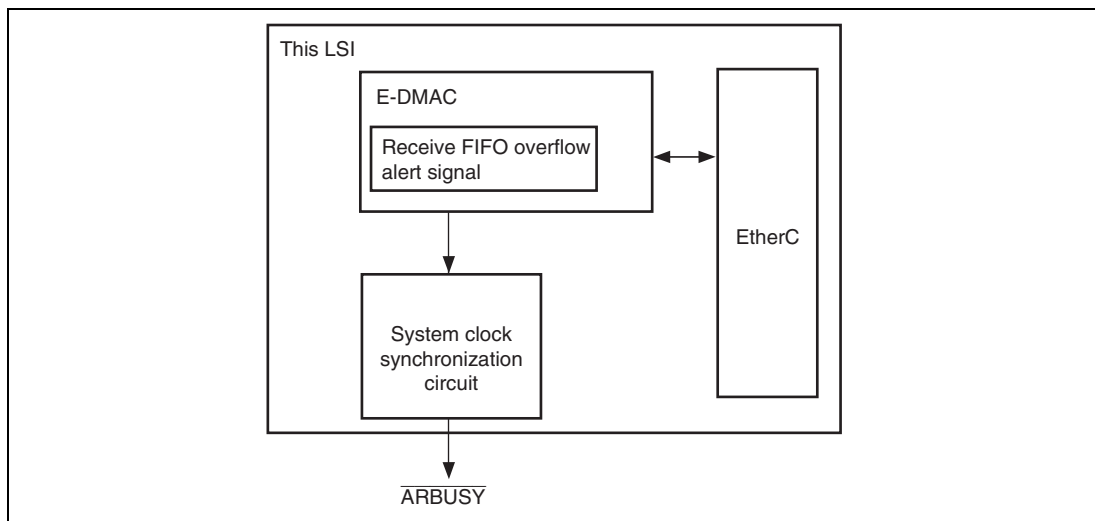
Figure 19.8 (2) Configuration of \overline{\text{ARBUSY}} (SH7713)
