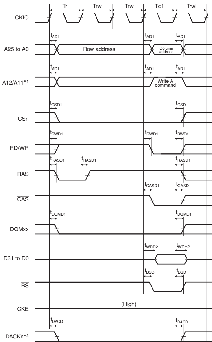
Figure 25.27 Synchronous DRAM Single Write Bus Cycle (Auto Precharge, WTRCD = 2 Cycle, TRWL = 1 Cycle)
