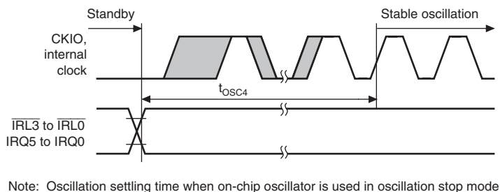
Figure 25.8 Oscillation Settling Time at Standby Return (Return by IRQ5 to IRQ0 and \overline{\text{IRL3}} to \overline{\text{IRL0}} )
