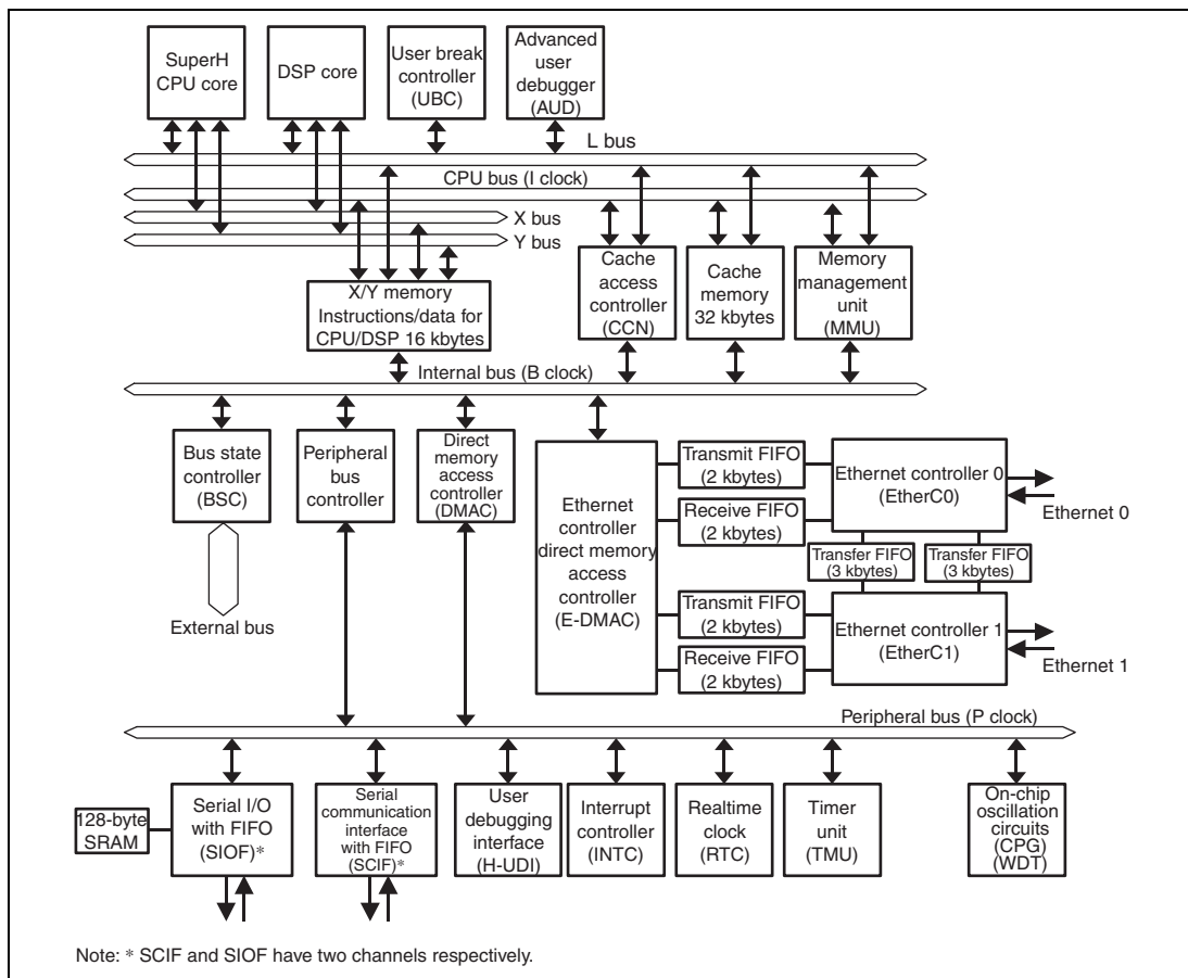
Figure 1.1 (2) Block Diagram (SH7712)
