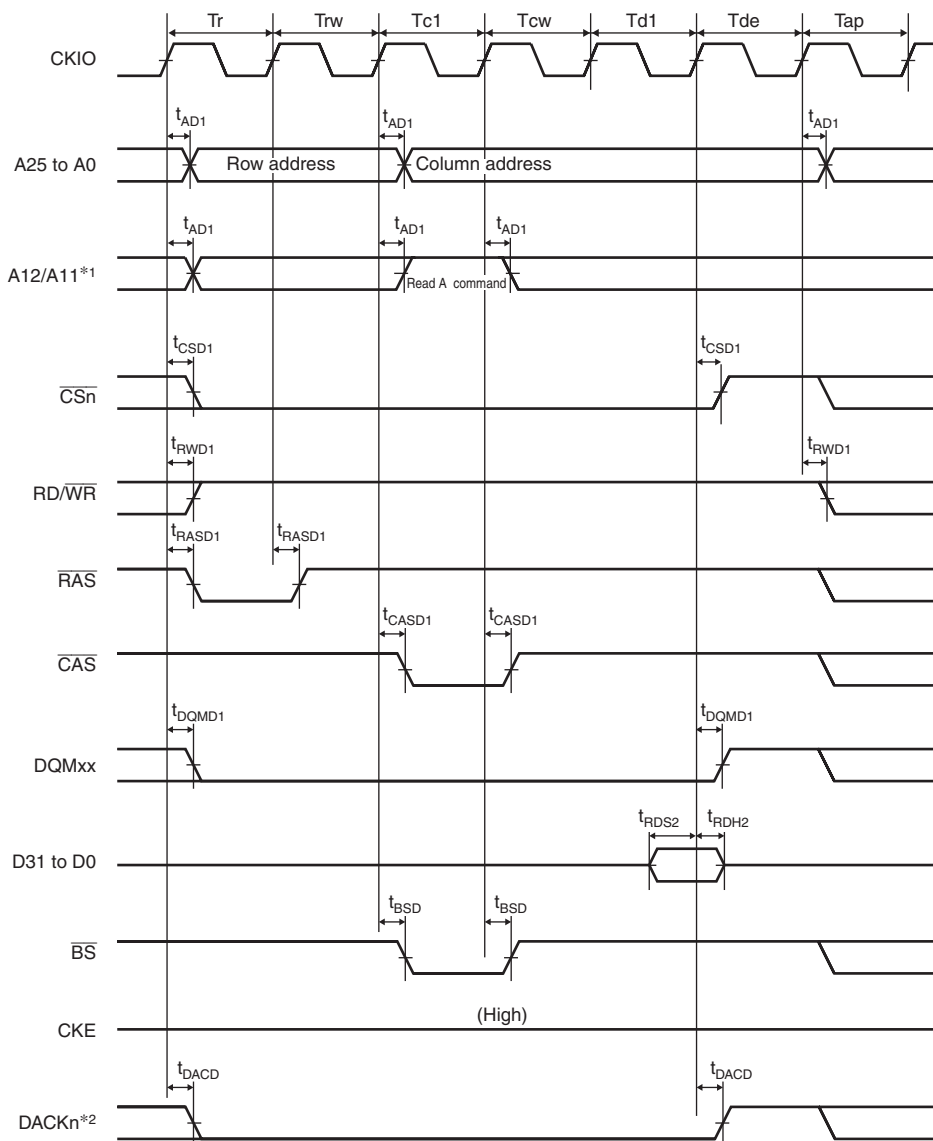
Figure 25.23 Synchronous DRAM Single Read Bus Cycle (Auto Precharge, CAS Latency = 2, WTRCD = 1 Cycle, WTRP = 1 Cycle)
