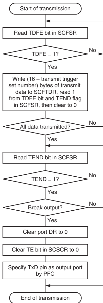
Figure 16.4 Sample Serial Transmission Flowchart
