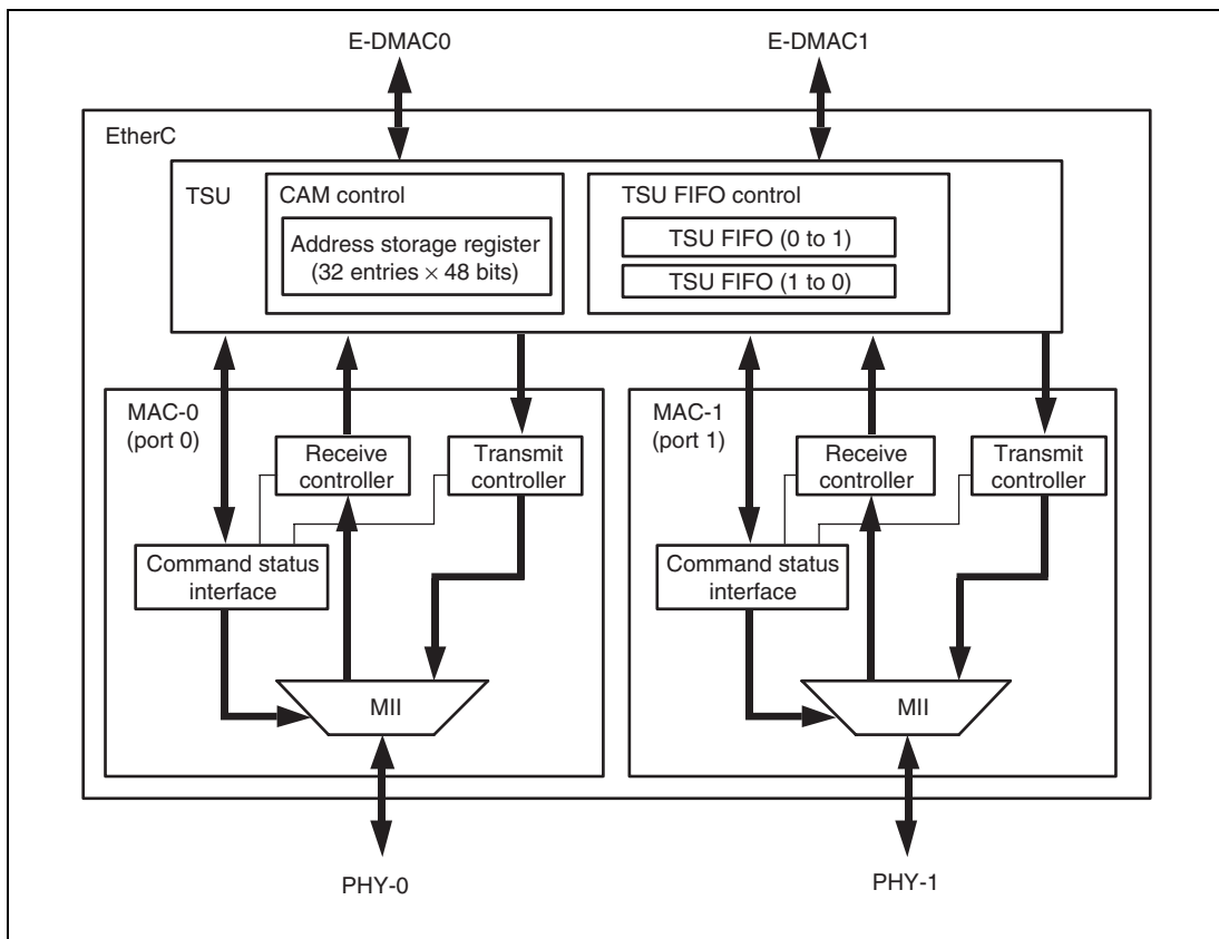
Figure 18.1 (1) Configuration of EtherC (SH7710, SH7712)
