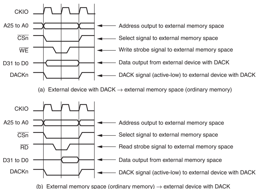
Figure 13.8 Example of DMA Transfer Timing in Single Address Mode
