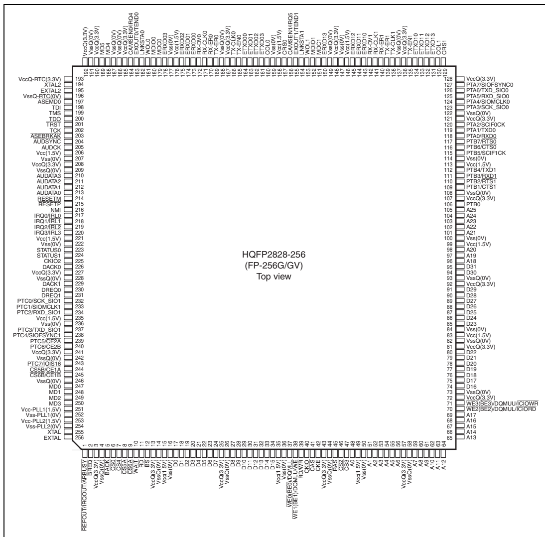
Figure 1.2 (1) Pin Assignment (HQFP2828-256 (FP-256G/GV)) (SH7710, SH7712)
