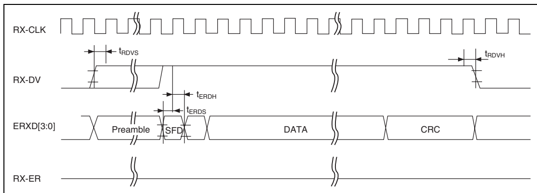
Figure 25.61 MII Receive Timing (Normal Operation)
