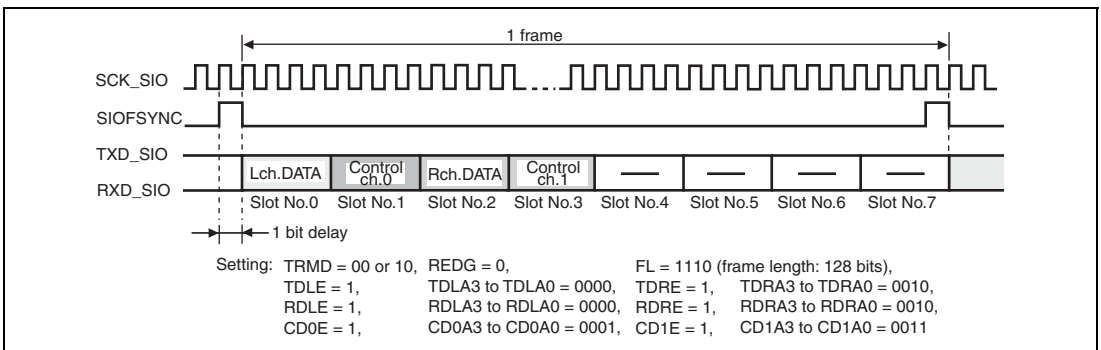
Figure 17.18 Transmission and Reception Timings (16-Bit Stereo Data (3))
