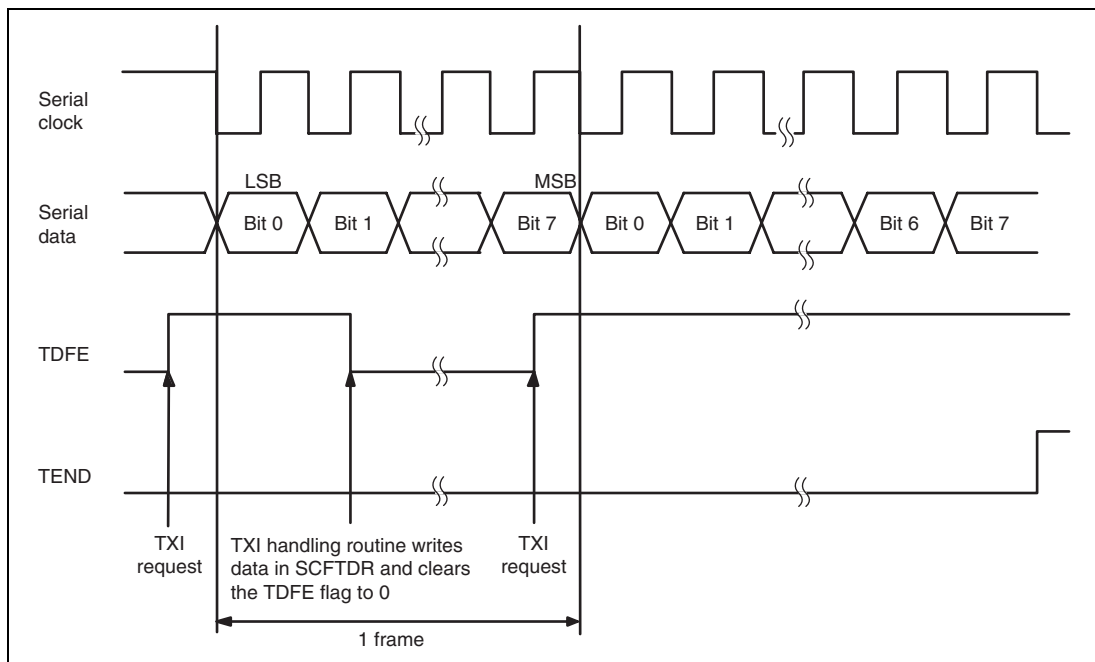
Figure 16.14 Example of the SCIF Transmit Operation
