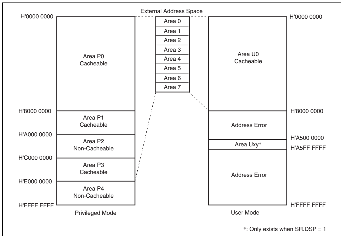
Figure 5.3 Virtual Address Space (MMUCR.AT = 0)
