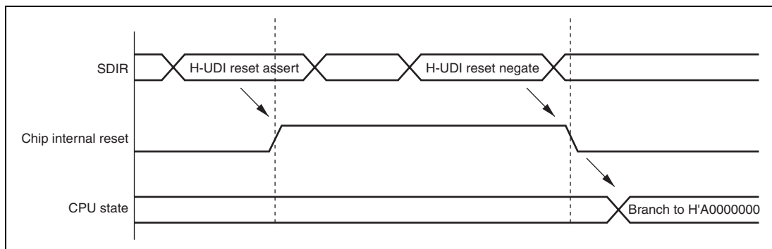
Figure 23.4 H-UDI Reset
