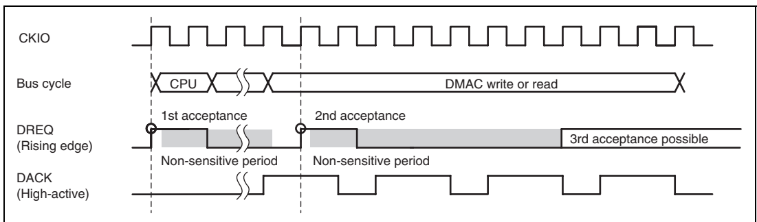
Figure 13.18 Example of DREQ Input Detection in Cycle Steal Mode Edge Detection When DACK is Divided to 4 by Idle Cycles
