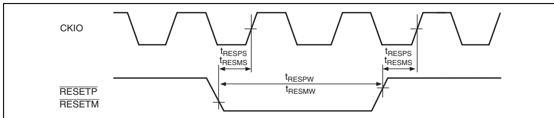
Figure 25.12 Reset Input Timing
