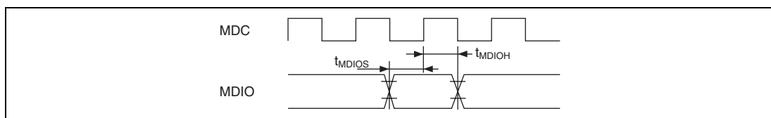
Figure 25.63 MDIO Input Timing
