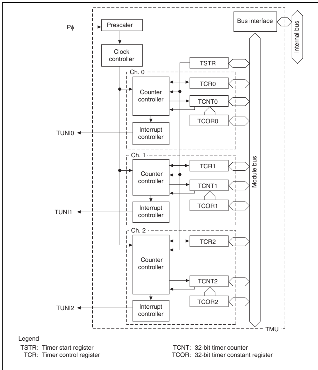
Figure 14.1 TMU Block Diagram
