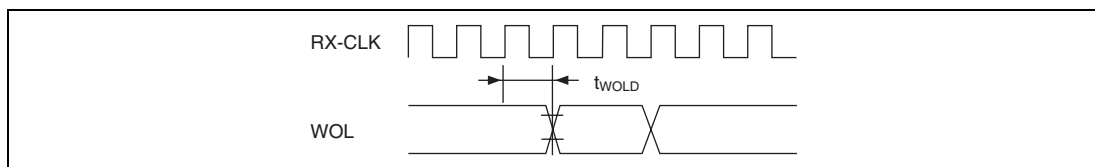
Figure 25.64 WOL Output Timing
