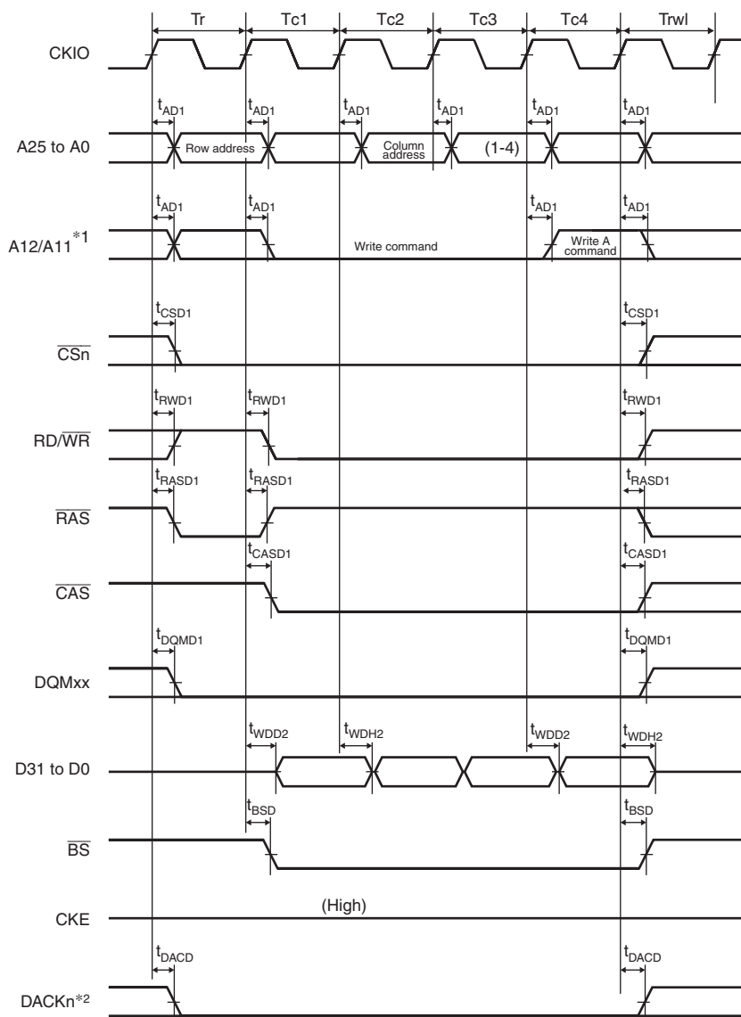
Figure 25.28 Synchronous DRAM Burst Write Bus Cycle (Single Write x 4), (Auto Precharge, WTRCD = 0 Cycle, TRWL = 1 Cycle)
