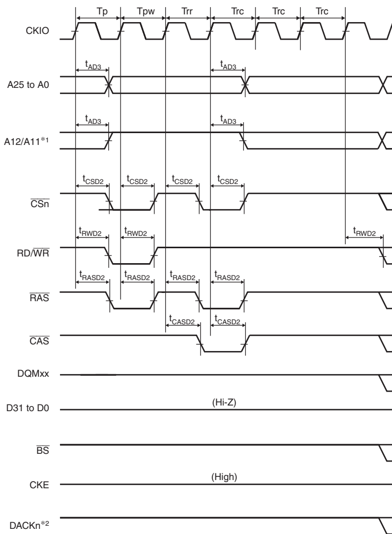
Figure 25.45 Synchronous DRAM Auto-Refresh Timing (WTRP = 1 Cycle, Low-Frequency Mode)
