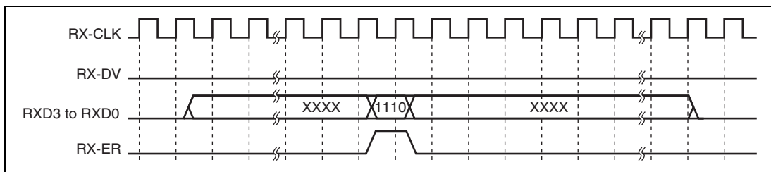
Figure 18.7 (6) MII Fame Receive Timing (Reception Error (2))
