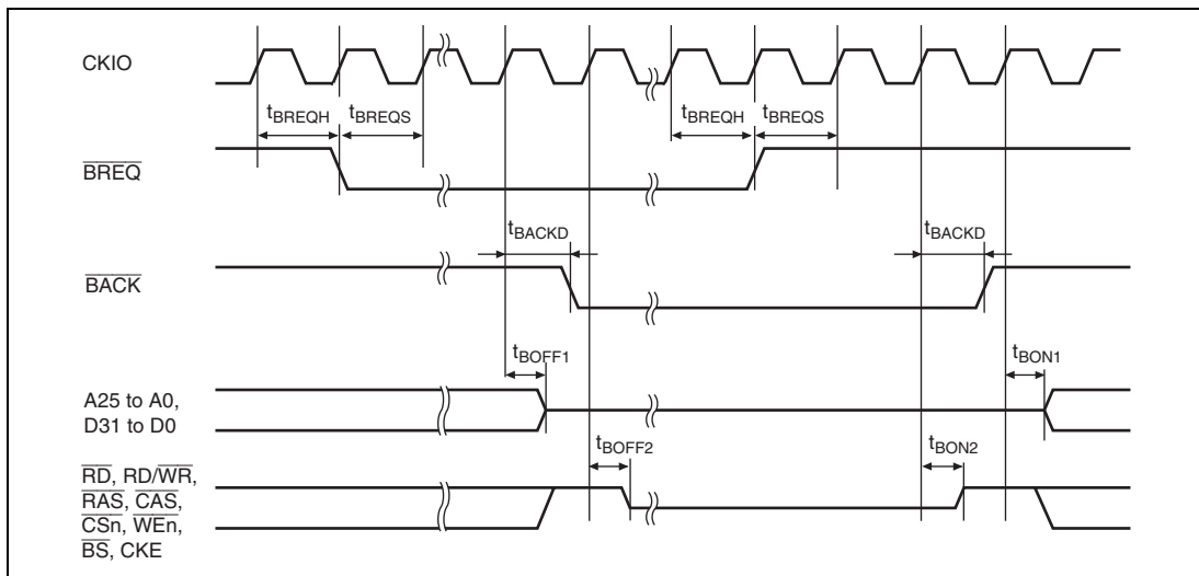
Figure 25.14 Bus Release Timing
