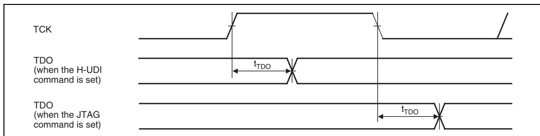
Figure 23.3 H-UDI Data Transfer Timing
