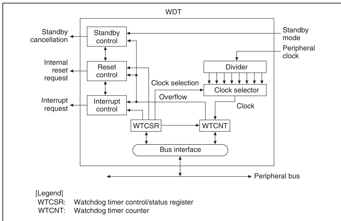
Figure 11.2 Block Diagram of WDT
