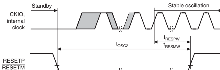
Figure 25.5 Power-On Oscillation Settling Time
