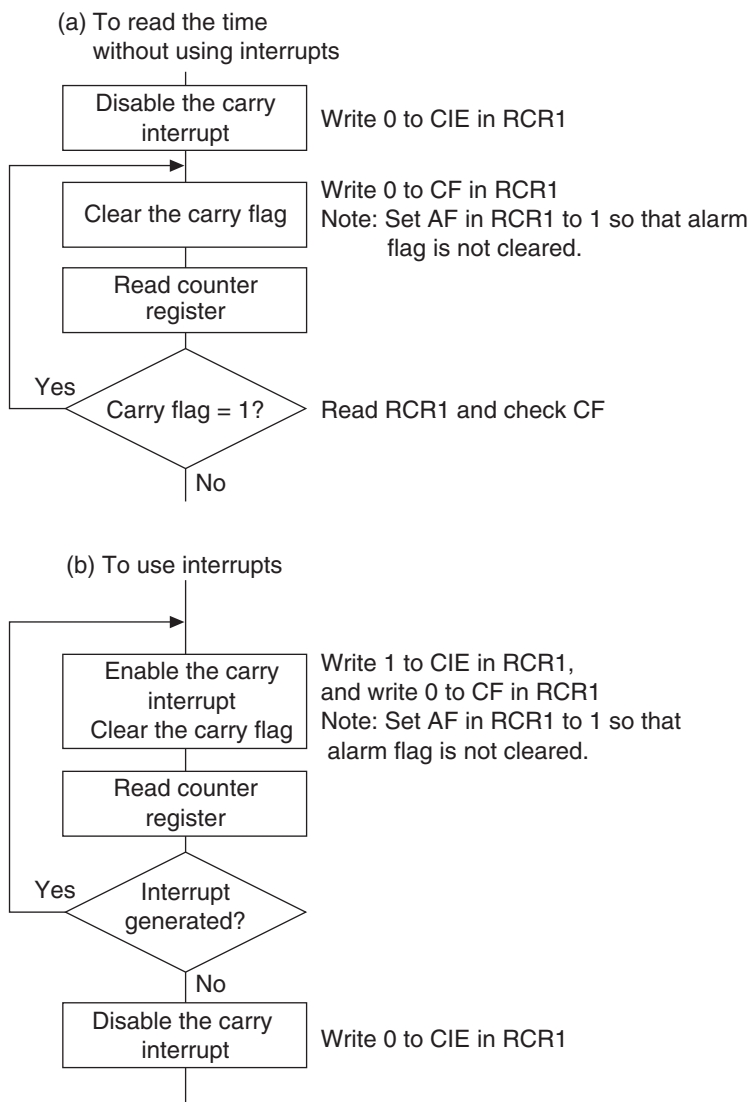
Figure 15.3 Reading Time
