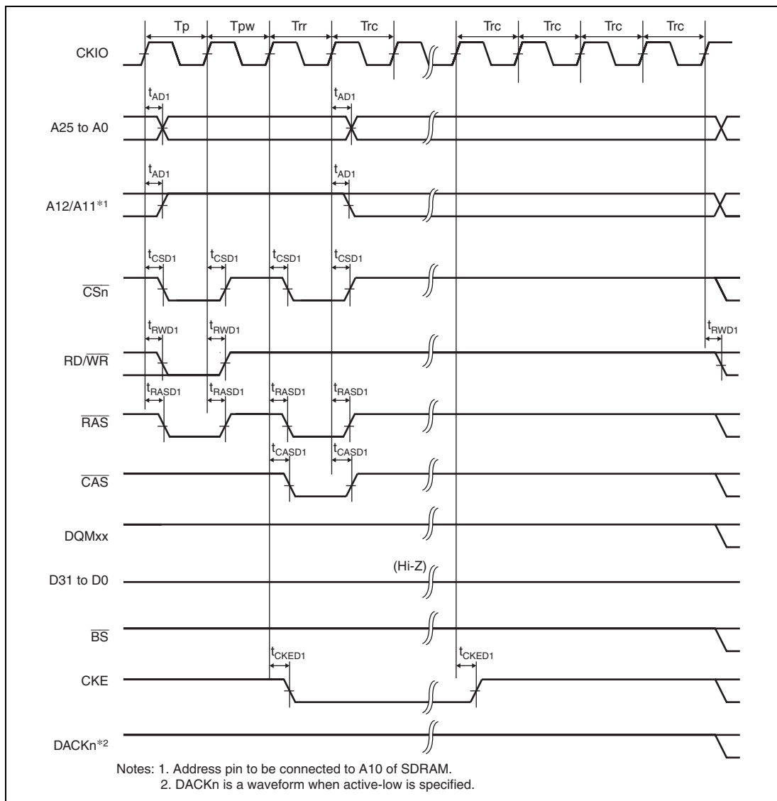
Figure 25.37 Synchronous DRAM Self-Refresh Timing (WTRP = 1 Cycle)
