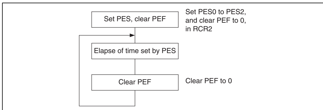
Figure 15.6 Using Periodic Interrupt Function
