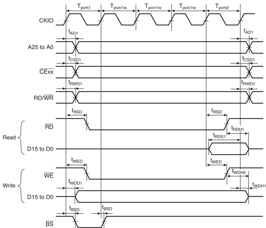
Figure 25.39 PCMCIA Memory Card Interface Bus Timing
