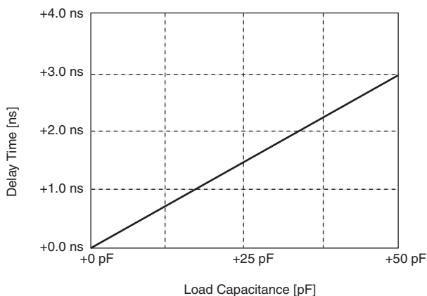
Figure 25.75 Load Capacitance vs. Delay Time
