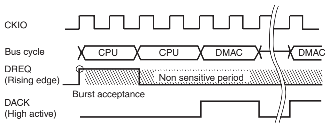
Figure 13.14 Example of DREQ Input Detection in Burst Mode Edge Detection
