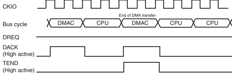
Figure 13.16 Example of DMA Transfer End Timing (Cycle Steal Level Detection)
