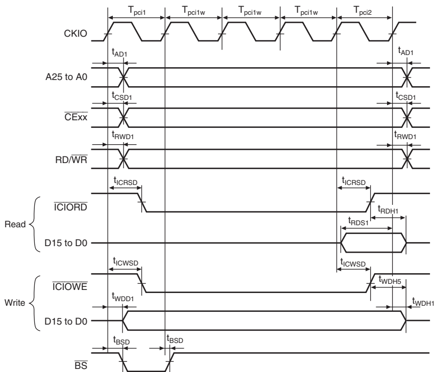
Figure 25.41 PCMCIA I/O Card Interface Bus Timing
