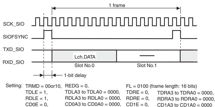
Figure 17.14 Transmission and Reception Timings (8-Bit Monaural Data (2))
