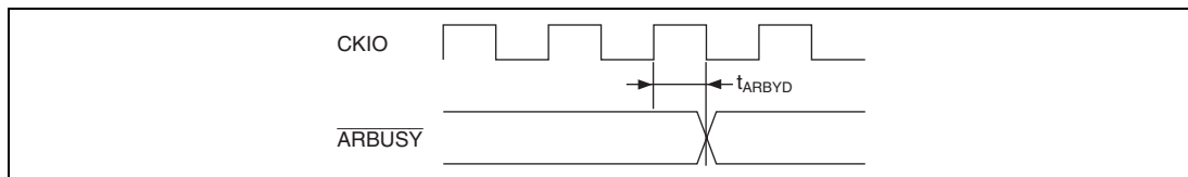
Figure 25.67 ARBUBY Output Timing
