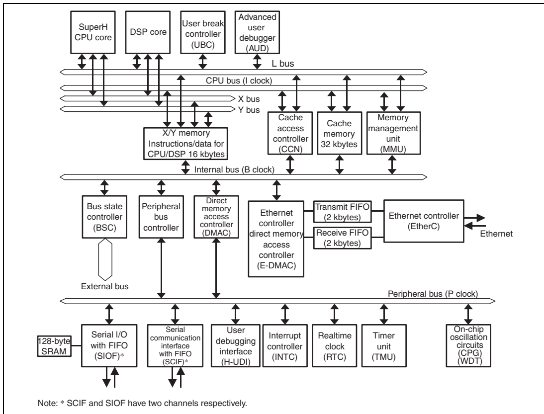
Figure 1.1 (3) Block Diagram (SH7713)
