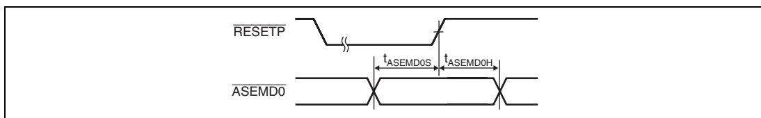
Figure 25.72 \overline{\text{ASEMD0}} Input Timing
