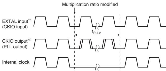
Figure 25.10 PLL Synchronization Settling Time by IRQ/IRL Interrupts
