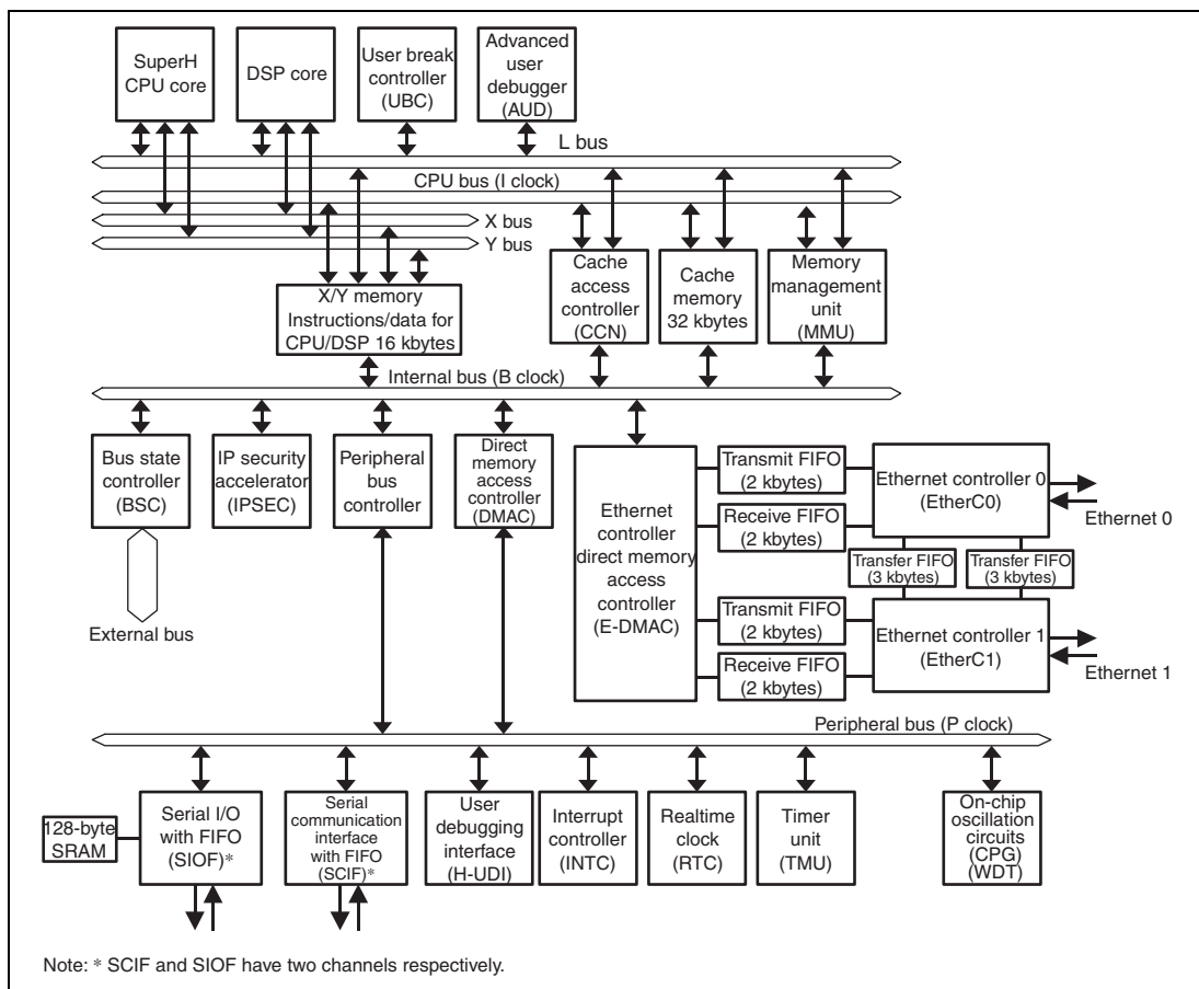
Figure 1.1 (1) Block Diagram (SH7710)
