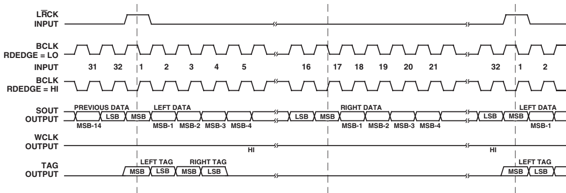
Figure 15. Serial Data Output Timing: Slave Mode, Left-Justified with No MSB Delay, 32-Bit Frame Mode, \overline{S\text{M}} = \text{HI} , \overline{R\text{LJUST}} = \text{LO} , \overline{\text{MSBDLY}} = \text{HI}
