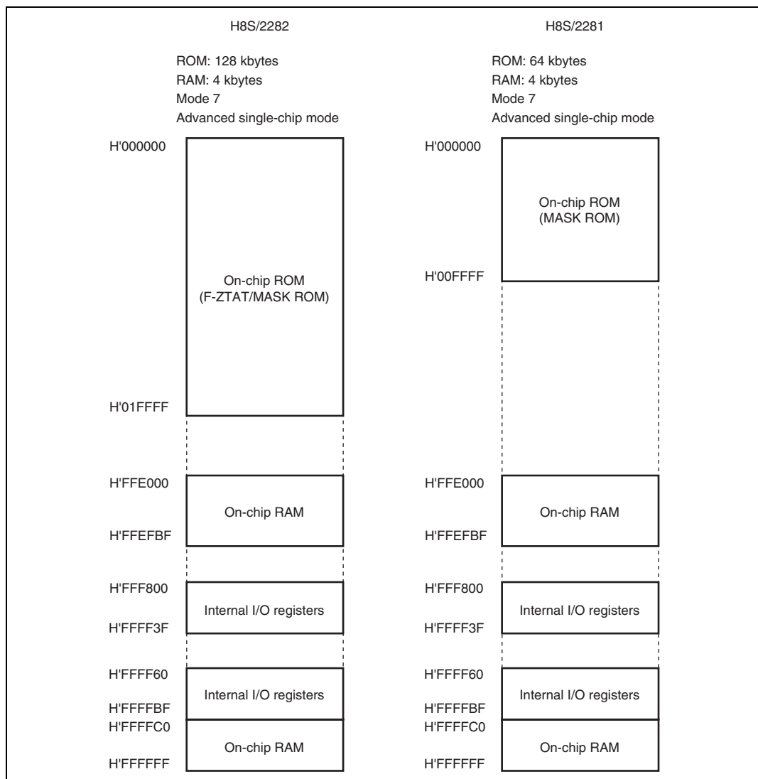
Figure 3.1 Address Map
