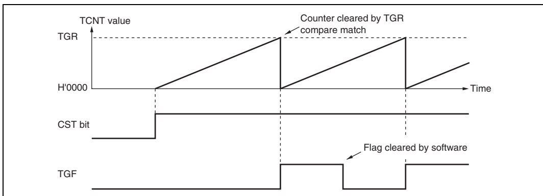
Figure 8.4 Periodic Counter Operation
