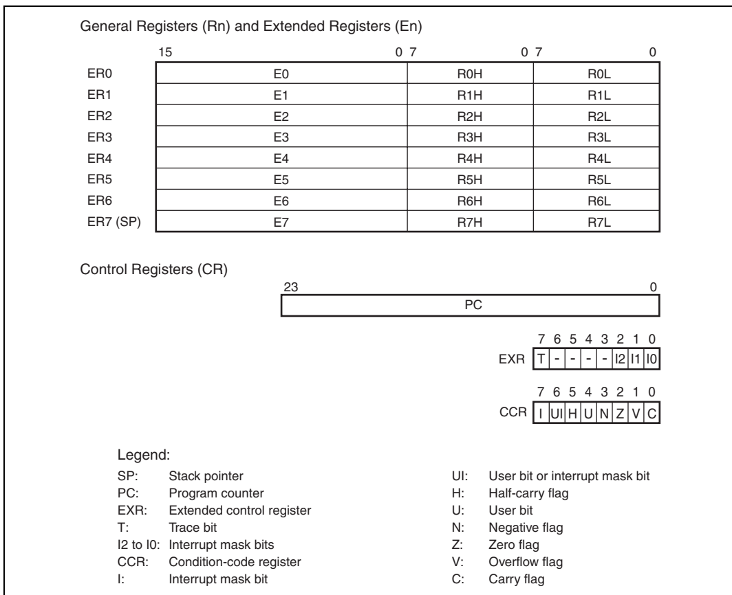
Figure 2.6 CPU Registers
