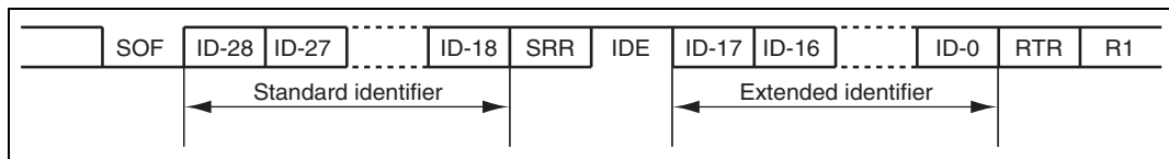
Figure 11.4 Extended Format
