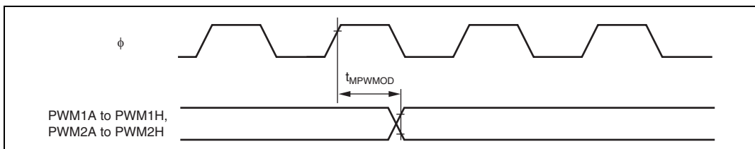
Figure 22.13 Motor Control PWM Output Timing
