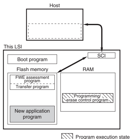
Figure 16.4 User Program Mode
