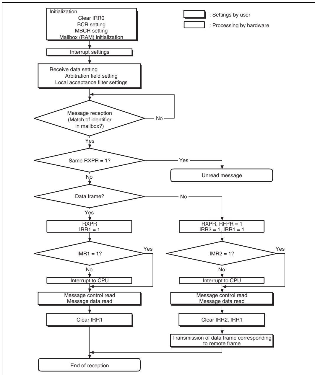
Figure 11.11 Reception Flowchart
