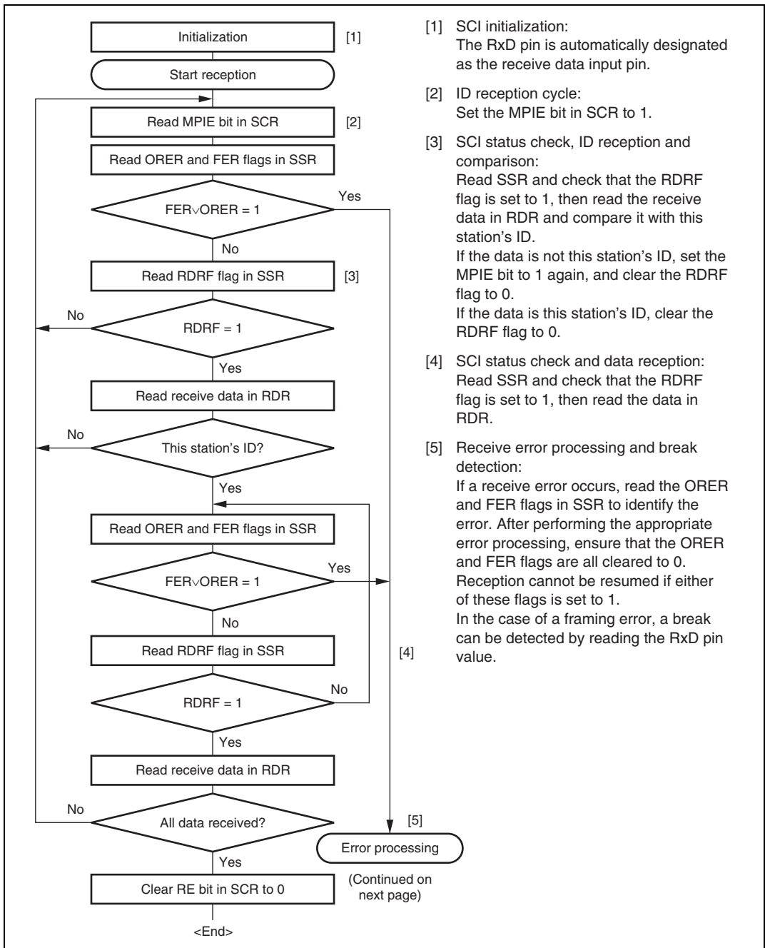
Figure 10.13 Sample Multiprocessor Serial Reception Flowchart (1)
