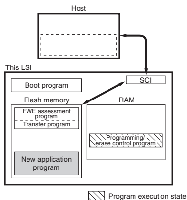
Figure 17.4 User Program Mode
