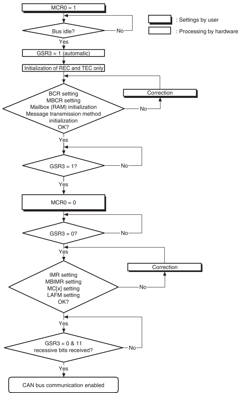
Figure 11.7 Software Reset Flowchart
