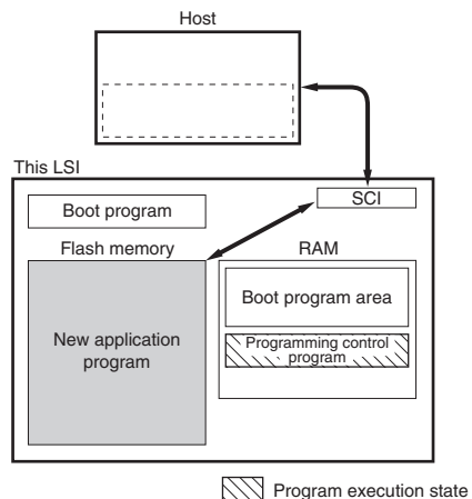
Figure 17.3 Boot Mode
