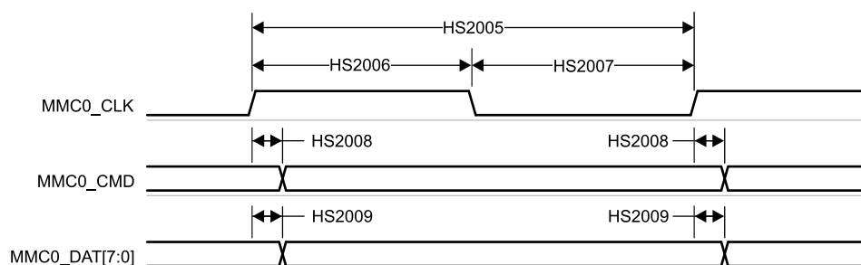
Figure 7-64. MMC0 – HS200 Mode – Transmit Mode
