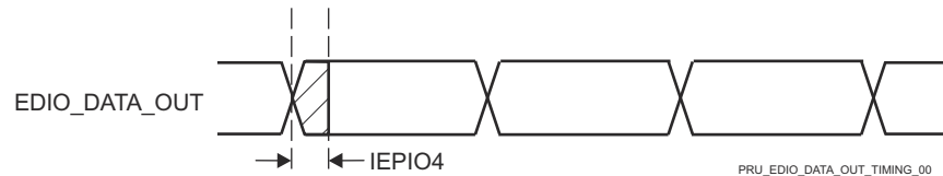
Figure 7-101. PRU_ICSSG IEP Digital IOs Timing Requirements
