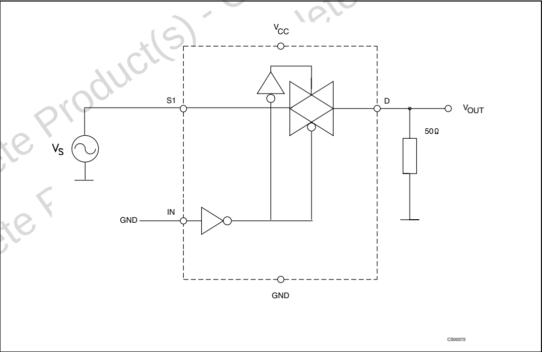
Figure 5. OFF isolation
