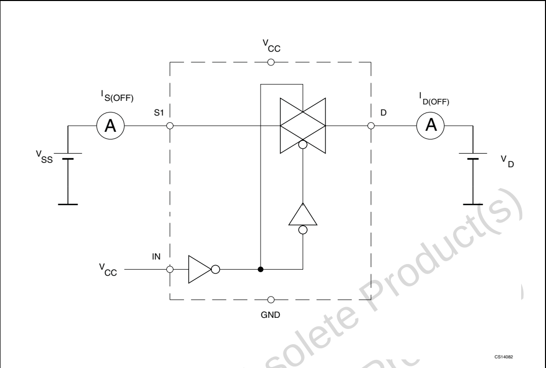
Figure 4. OFF leakage
