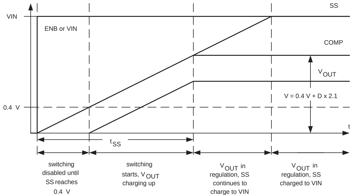
Figure 1. Waveforms During Softstart
