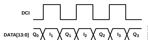
Figure 42. Timing Diagram for Word Mode
