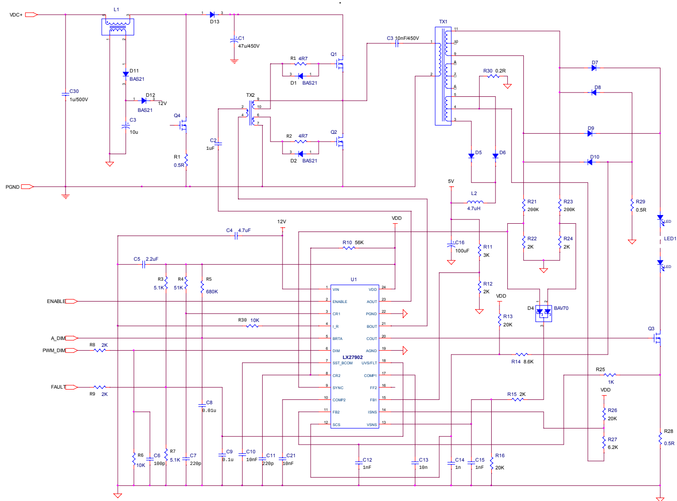
Figure 28 • Application Schematic, With Standby Power Management
