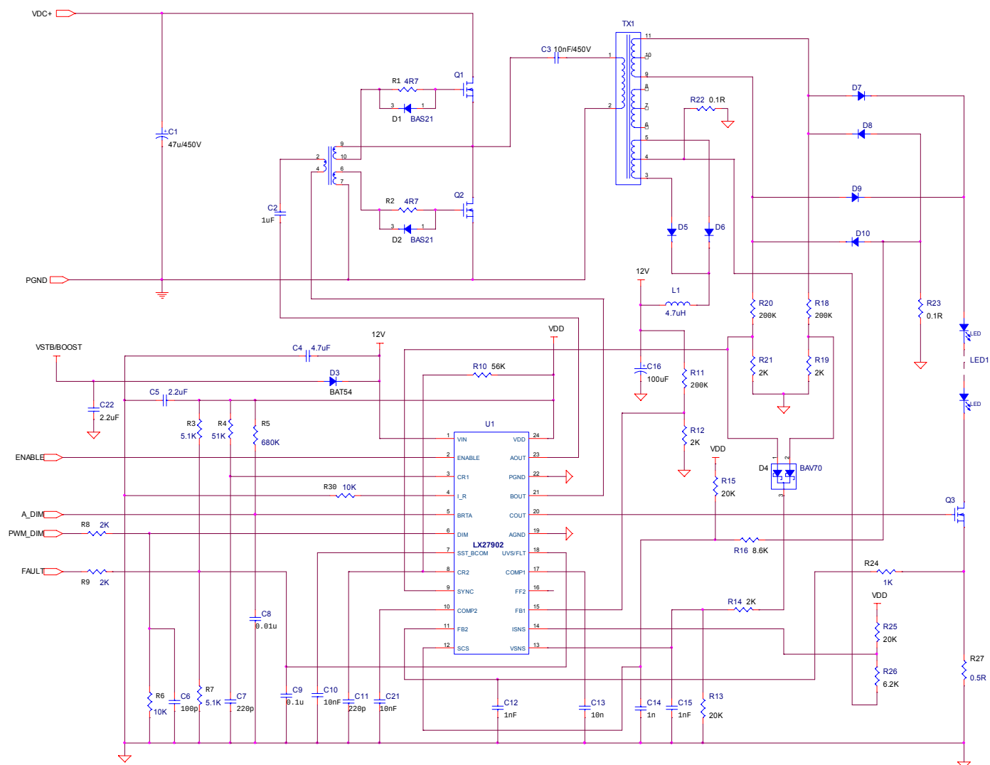
Figure 27 • Application Schematic
