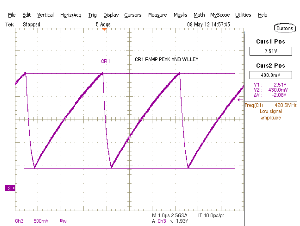
Figure 8 • CR1 Ramp Peak and Valley
