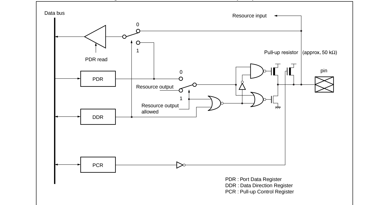
Figure PORT-2 Port block attached with a pullup resistor
