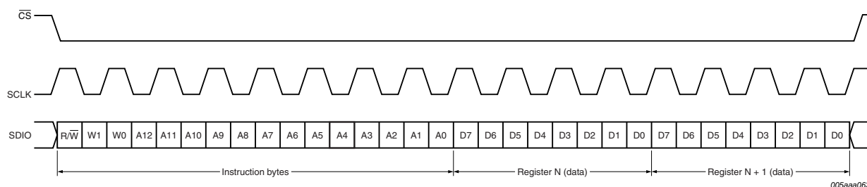
Fig 22. SPI mode timing
