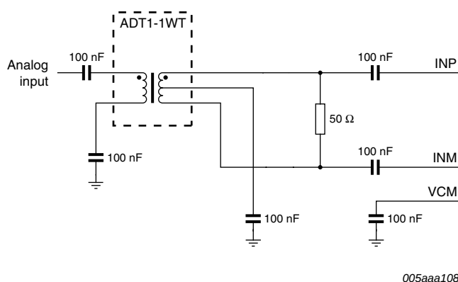
Fig 9. Single transformer configuration suitable for baseband applications
