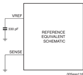
Fig 12. Internal reference, 2 V (p-p) full-scale
