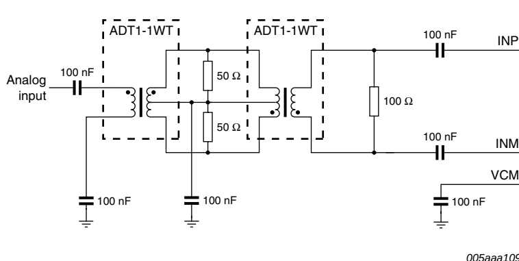
Fig 10. Dual transformer configuration suitable for high intermediate frequency application
