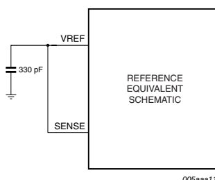
Fig 15. Internal reference via SPI, 1 V (p-p) to 2 V (p-p) full-scale
