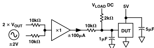
Figure 8a. Output Impedance Test Circuit
