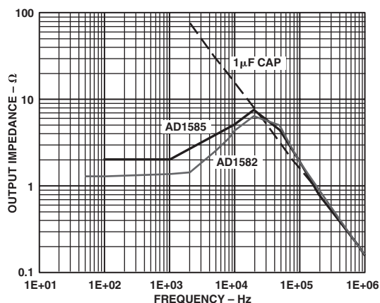
Figure 8b. Output Impedance vs. Frequency
