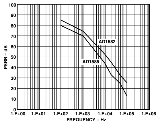
Figure 9b. Ripple Rejection vs. Frequency
