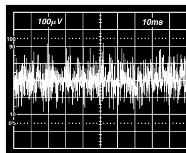
Figure 11. 10 Hz to 10 kHz Wideband Noise
