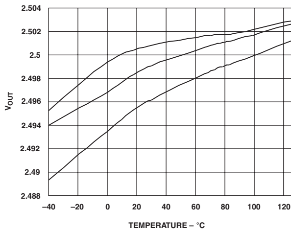
TPC 3. Typical Temperature Drift Characteristic Curves
