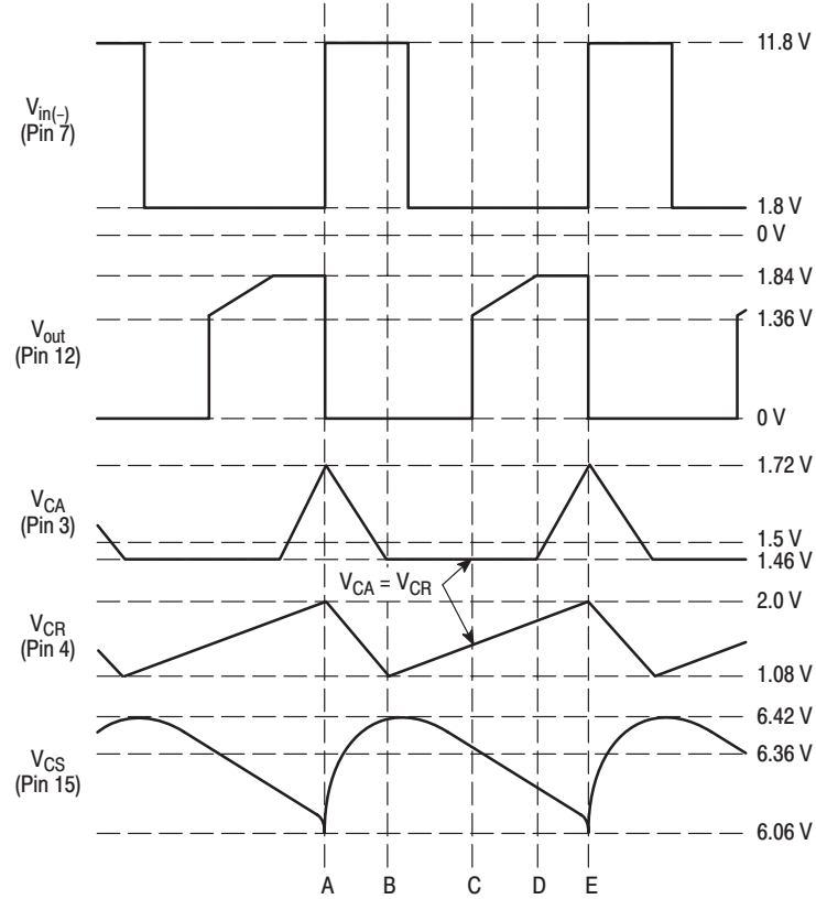
Figure 15. Run Mode 2000 RPM (Frequency: 66.67 Hz @ 5.0 ms)
