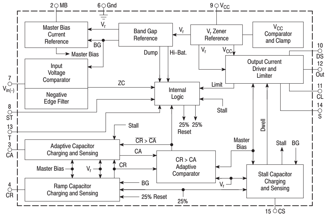
Figure 10. Block Diagram
