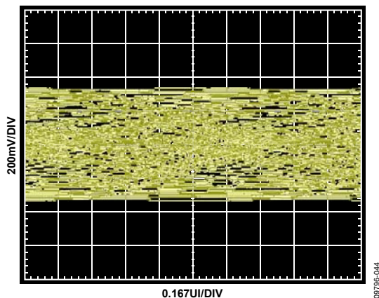
Figure 19. 4.25 Gbps Output Eye, 40-Inch FR4 Input Channel, PE = 0 dB (TP3 from Figure 17)
