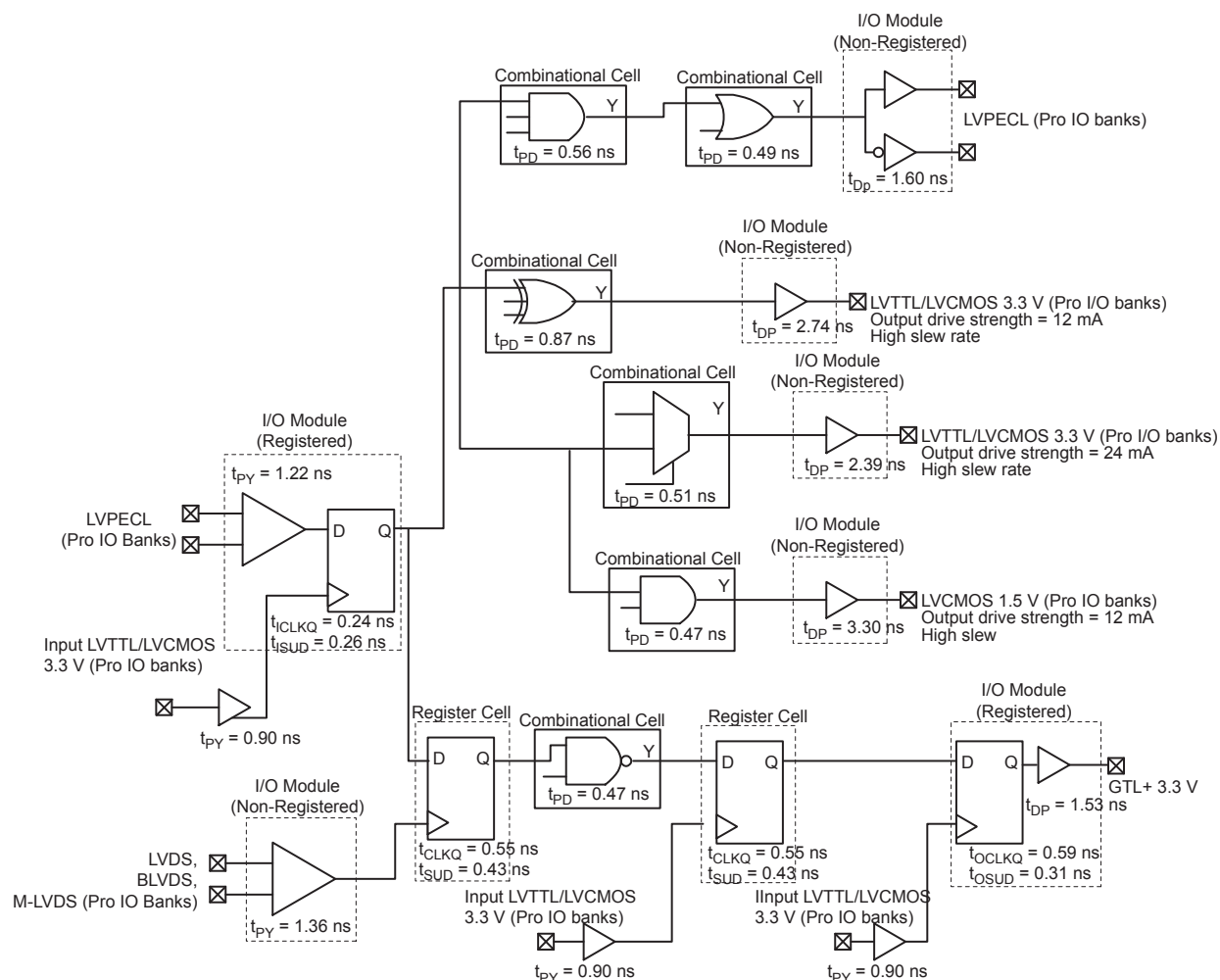
Figure 2-115 • Timing Model
