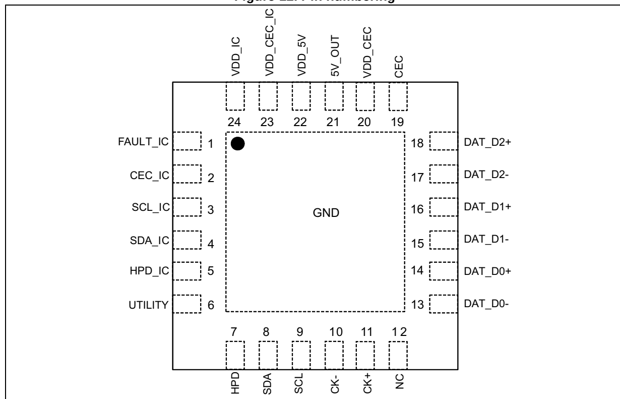
Figure 12. Pin numbering
