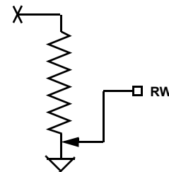
FIGURE 11. DCP CONNECTION IN SHUTDOWN MODE
