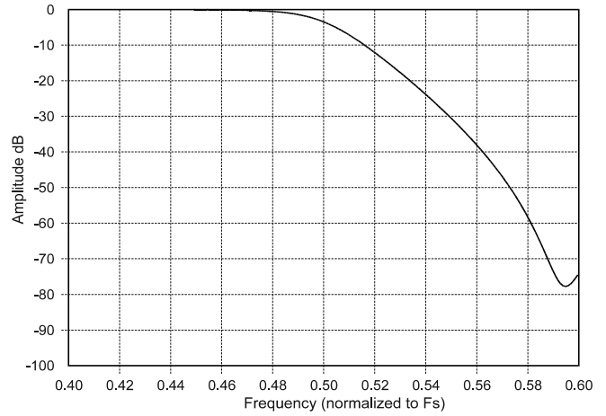
Figure 20. Transition Band
