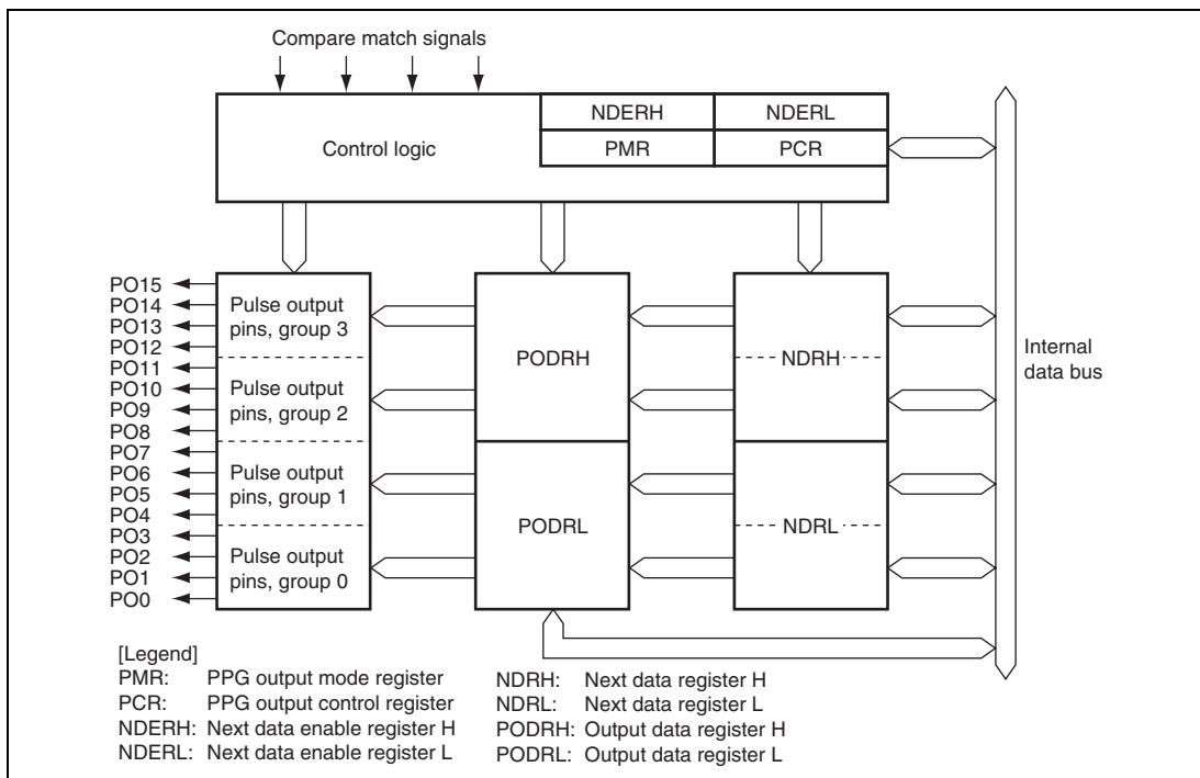
Figure 15.1 Block Diagram of PPG (Unit 0)
