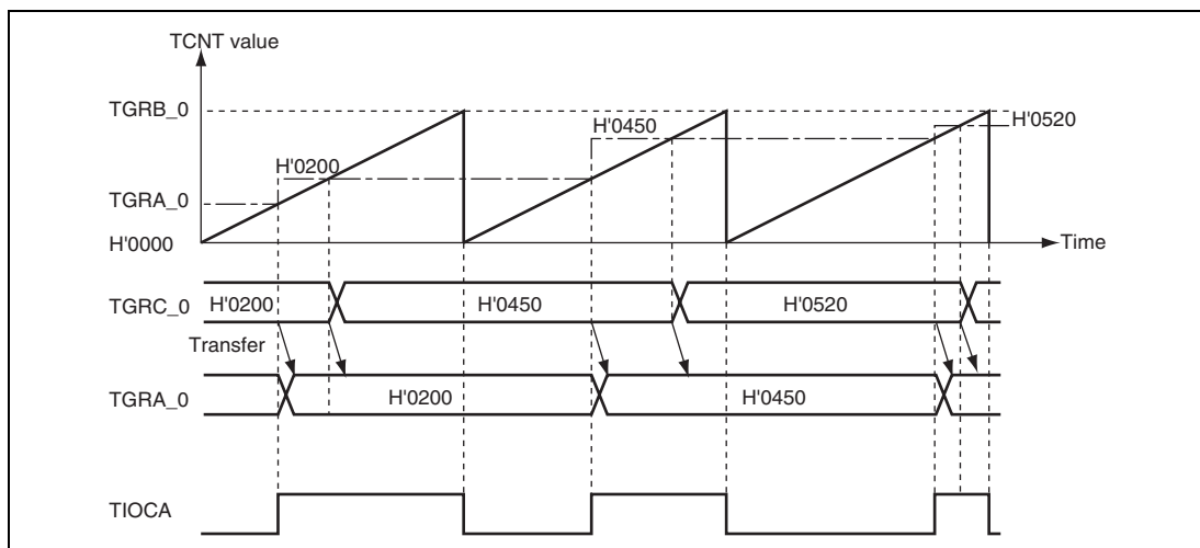
Figure 14.16 Example of Buffer Operation (1)
