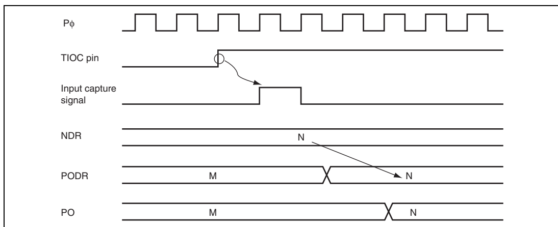
Figure 15.14 Pulse Output Triggered by Input Capture (Example)
