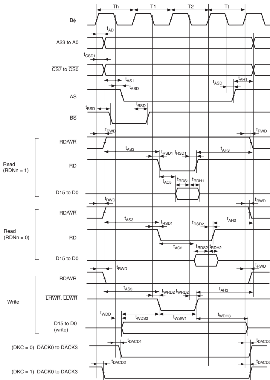
Figure 30.11 Basic Bus Timing: Two-State Access ( \overline{\text{CS}} Assertion Period Extended)
