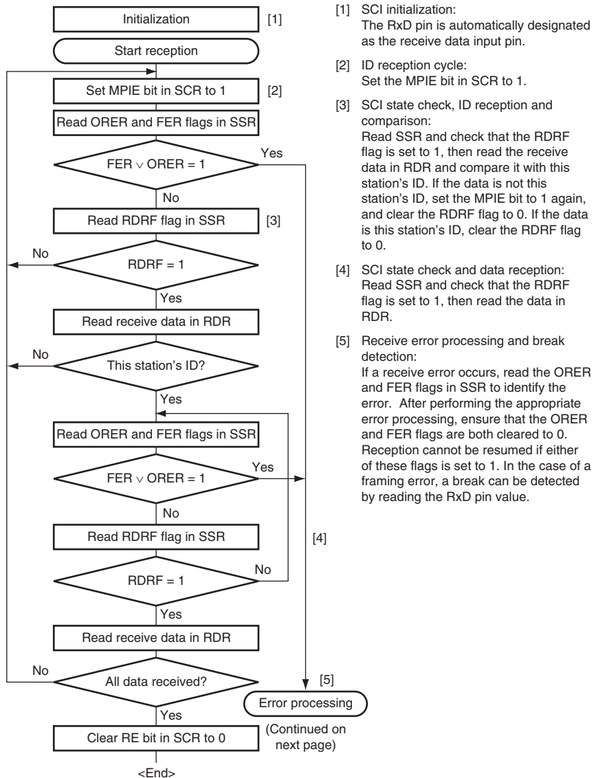
Figure 19.16 Sample Multiprocessor Serial Reception Flowchart (1)
