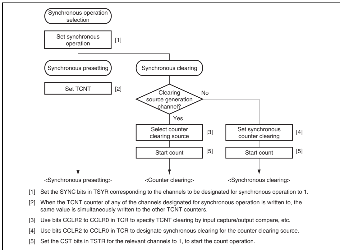
Figure 14.11 Example of Synchronous Operation Setting Procedure
