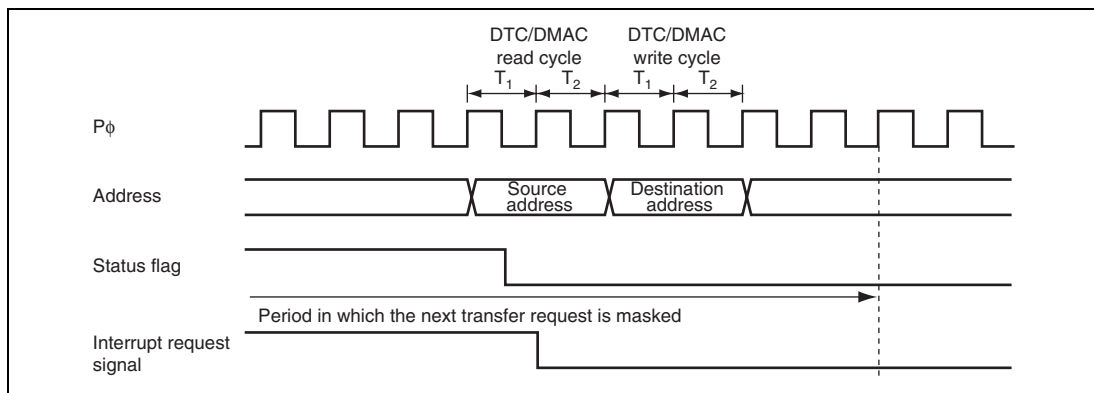
Figure 14.44 Timing for Status Flag Clearing by DTC/DMAC Activation (1)
