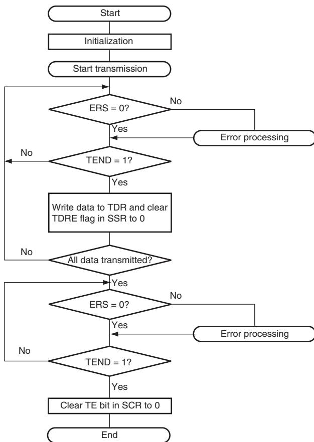
Figure 19.31 Sample Transmission Flowchart
