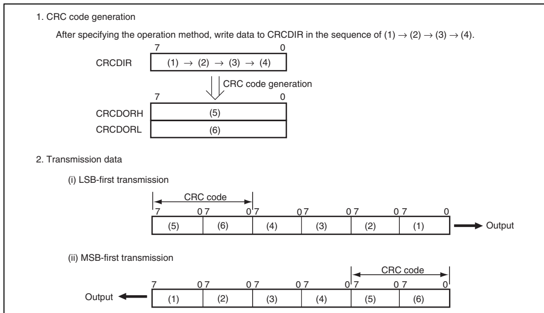
Figure 19.48 LSB-First and MSB-First Transmit Data
