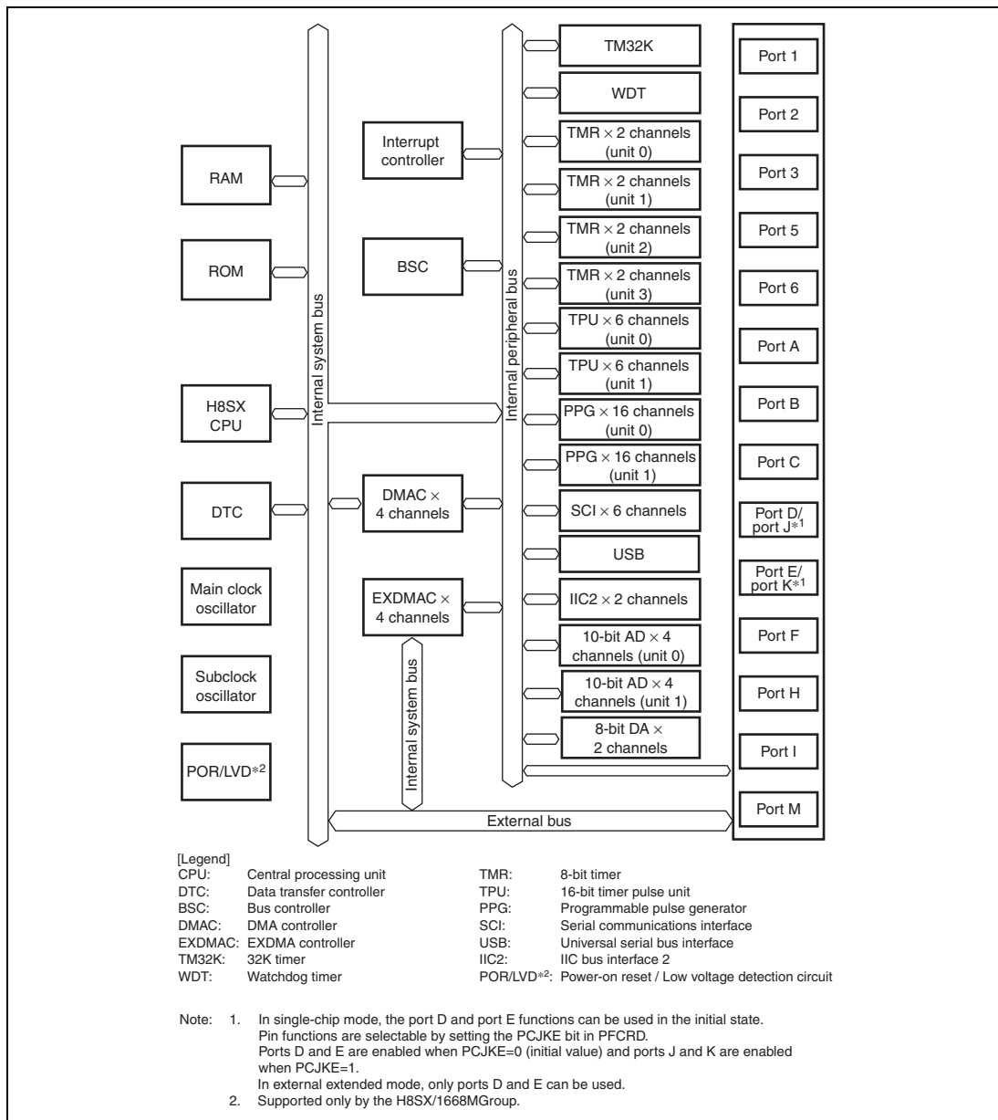
Figure 1.2 Block Diagram
