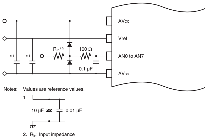
Figure 22.13 Example of Analog Input Protection Circuit
