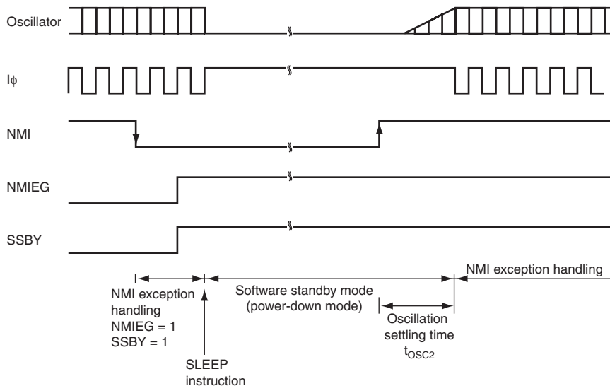
Figure 30.3 Oscillation Settling Timing after Software Standby Mode
