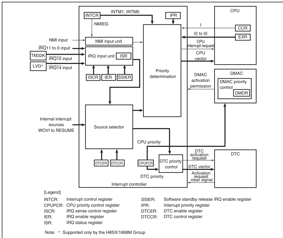
Figure 7.1 Block Diagram of Interrupt Controller
