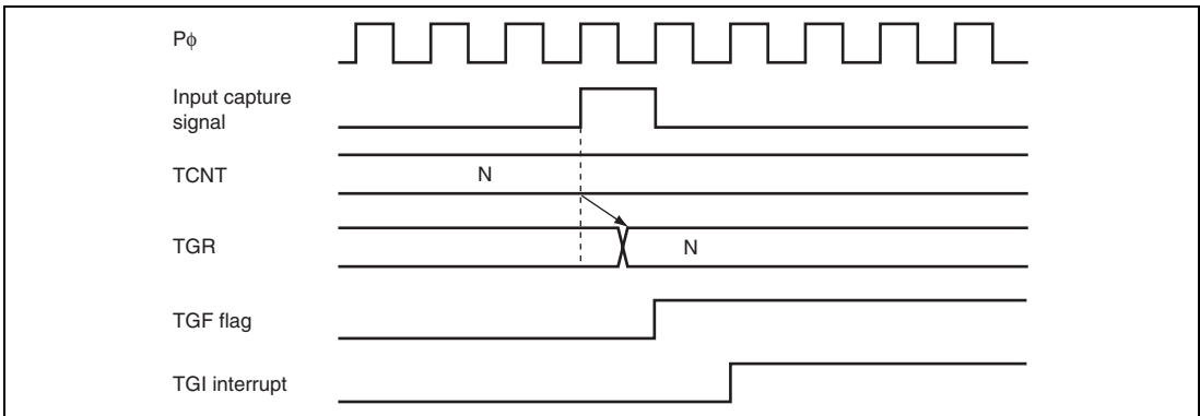
Figure 14.40 TGI Interrupt Timing (Input Capture)
