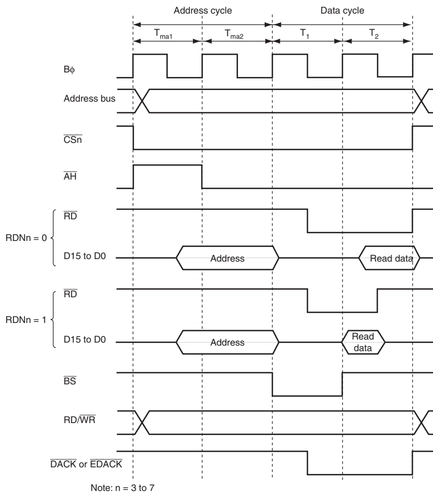
Figure 9.34 Read Strobe Timing
