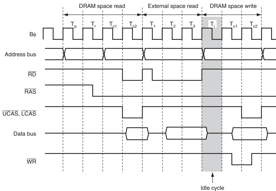
Figure 9.101 Example of Idle Cycles in RAS Down Mode (Write after Read)
