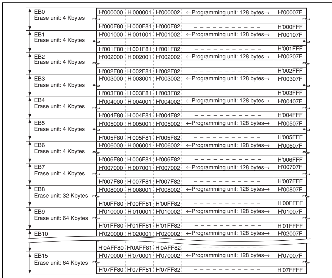
Figure 25.4 (2) User MAT Block Structure of H8SX/1664
