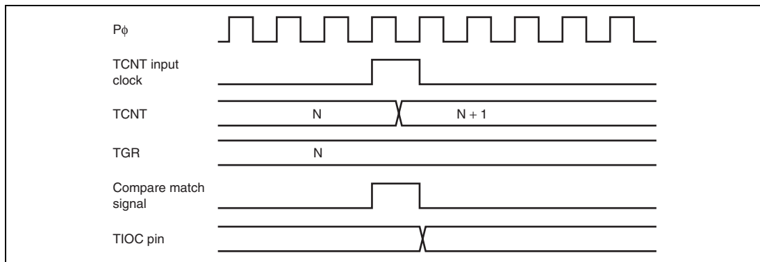
Figure 14.33 Output Compare Output Timing
