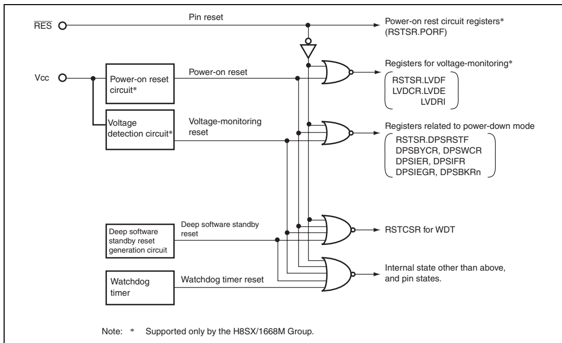
Figure 4.1 Block Diagram of Reset Circuit
