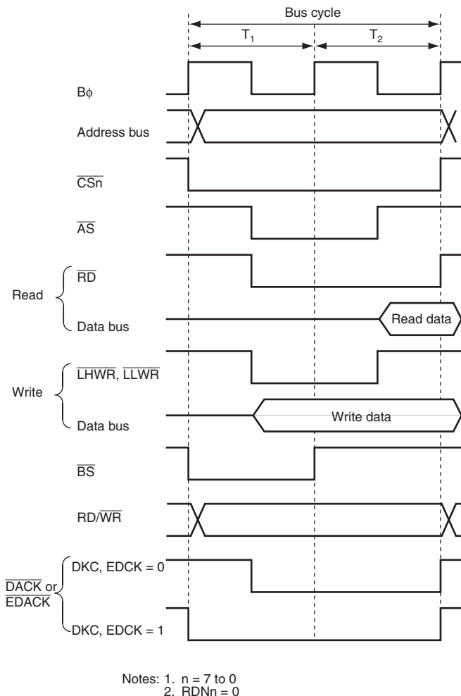
Figure 9.24 \overline{\text{DACK}} and \overline{\text{EDACK}} Signal Output Timing
