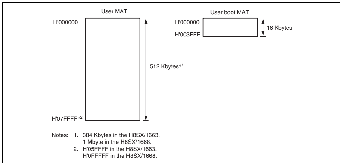
Figure 25.3 Memory MAT Configuration (H8SX/1644)
