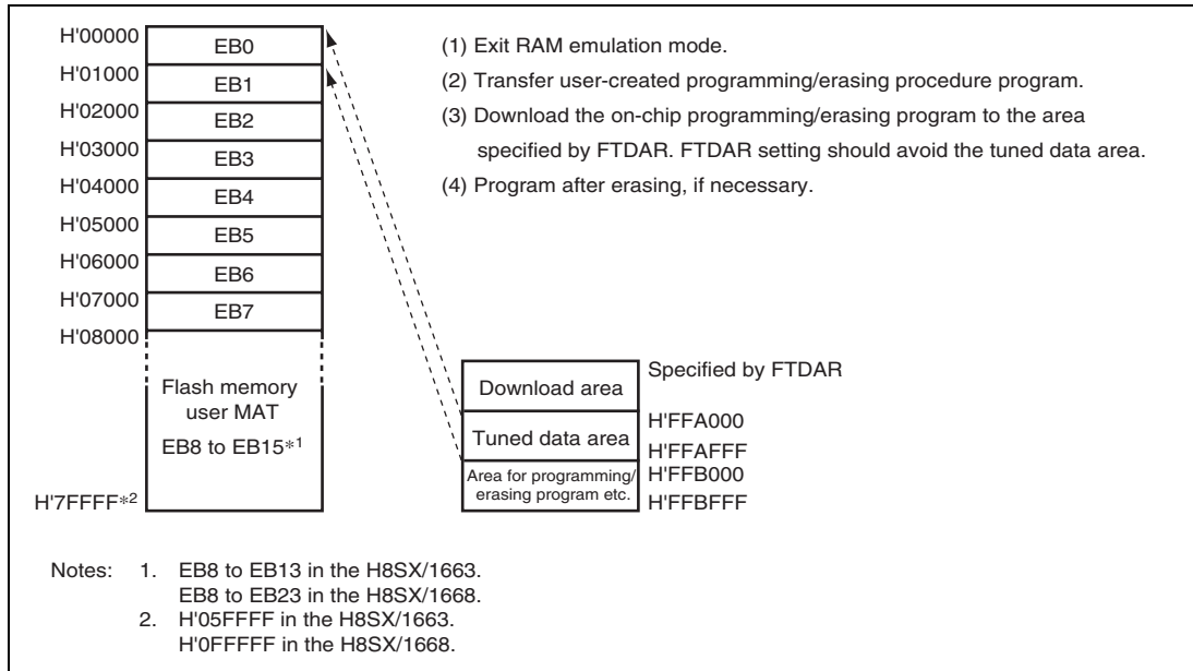
Figure 25.21 Programming Tuned Data (H8SX/1664)
