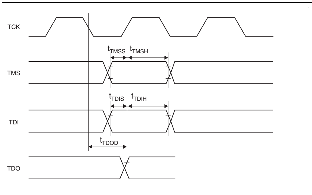
Figure 30.56 Boundary Scan Input/Output Timing
