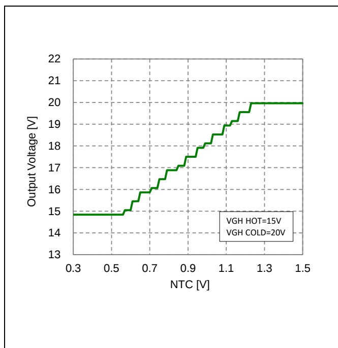
Figure 50. NTC Function (VGH)
