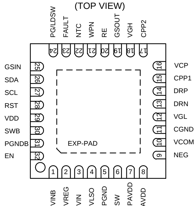
Figure 2. Pin Configuration
