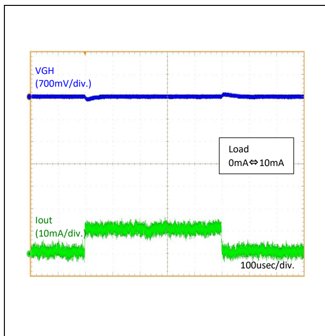
Figure 48. Load Transient (VGH)
