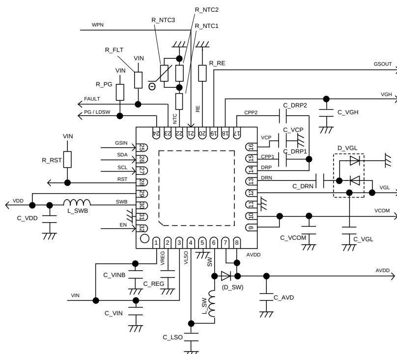
Figure 1. Application Circuit
