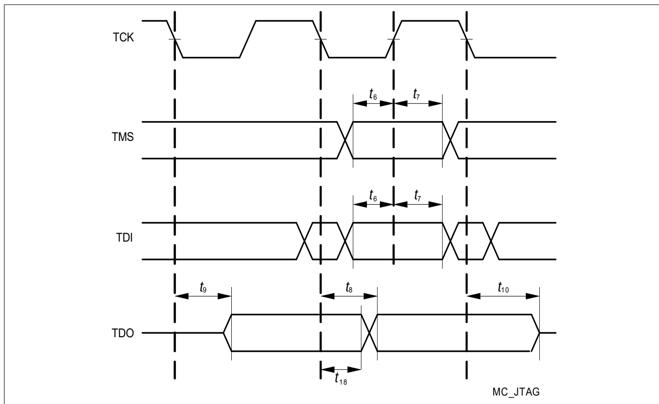
Figure 3-11 JTAG Timing
